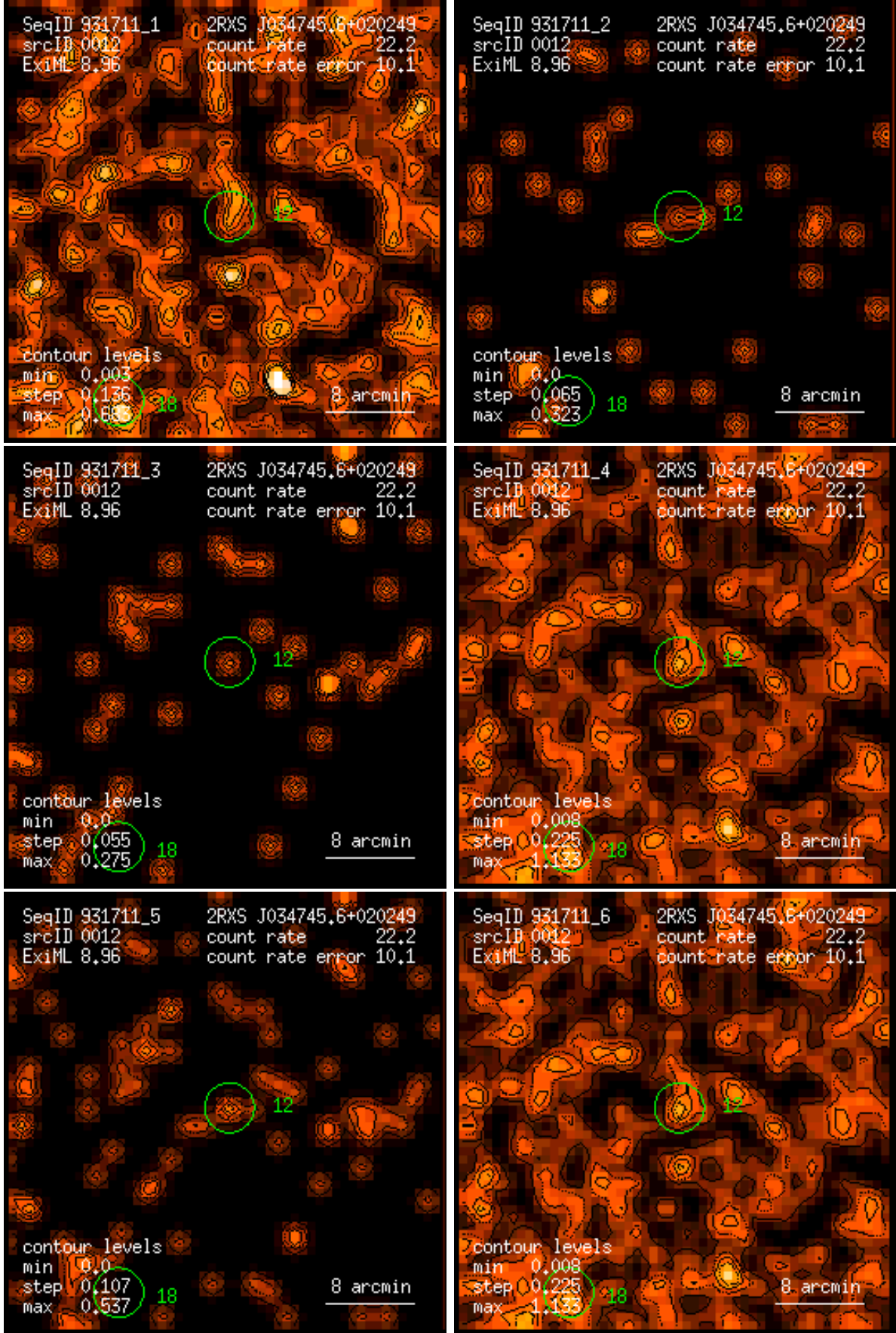
Figure 12: RASS 931711: detection 0012: band rate images, Gaussian filter: (1) PSPC channels 11 – 41, (2) 52 – 90, (3) 91 – 201, (4) 11 – 235, (5) 52 – 201, (6) 11 – 201. Broad band rates in counts/ks. Band rate contour levels in counts/ks/arcmin 2 .
