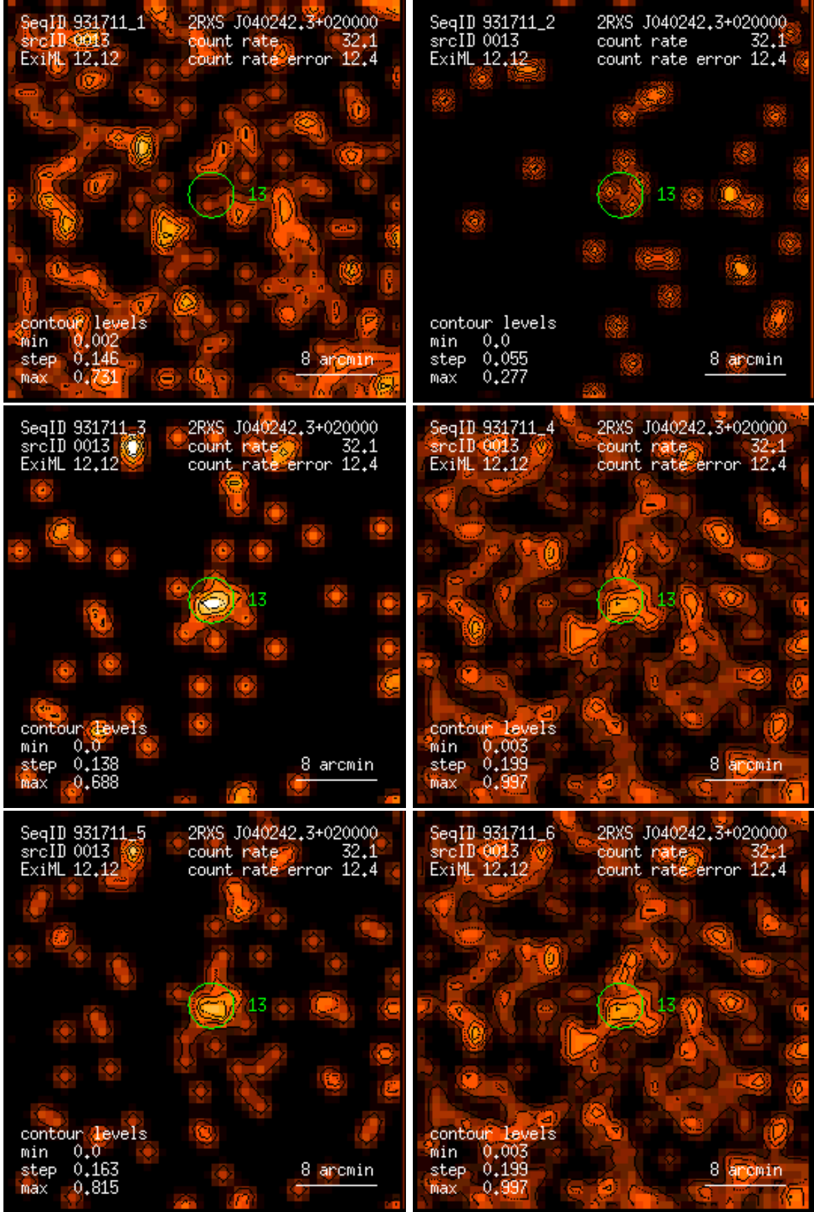
Figure 13: RASS 931711: detection 0013: band rate images, Gaussian filter: (1) PSPC channels 11 – 41, (2) 52 – 90, (3) 91 – 201, (4) 11 – 235, (5) 52 – 201, (6) 11 – 201. Broad band rates in counts/ks. Band rate contour levels in counts/ks/arcmin 2 .
