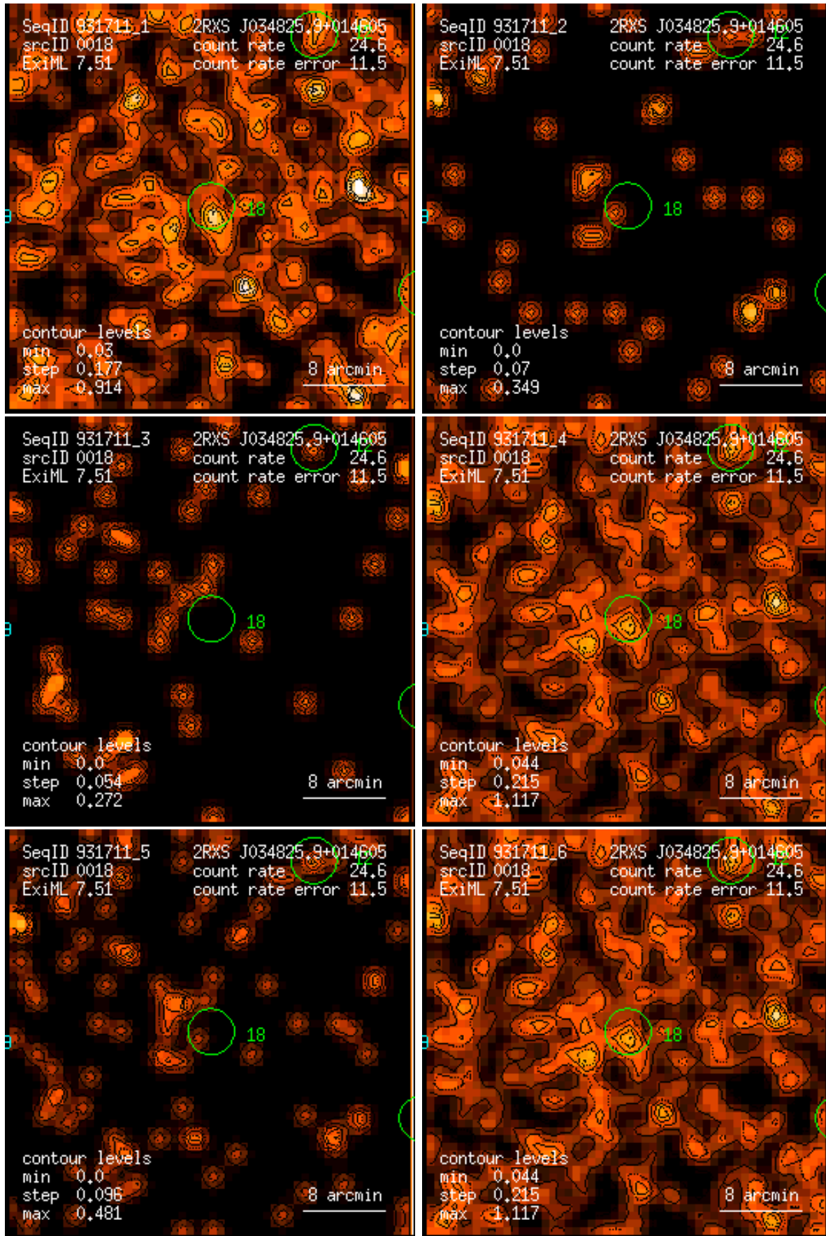
Figure 18: RASS 931711: detection 0018: band rate images, Gaussian filter: (1) PSPC channels 11 – 41, (2) 52 – 90, (3) 91 – 201, (4) 11 – 235, (5) 52 – 201, (6) 11 – 201. Broad band rates in counts/ks. Band rate contour levels in counts/ks/arcmin 2 .
