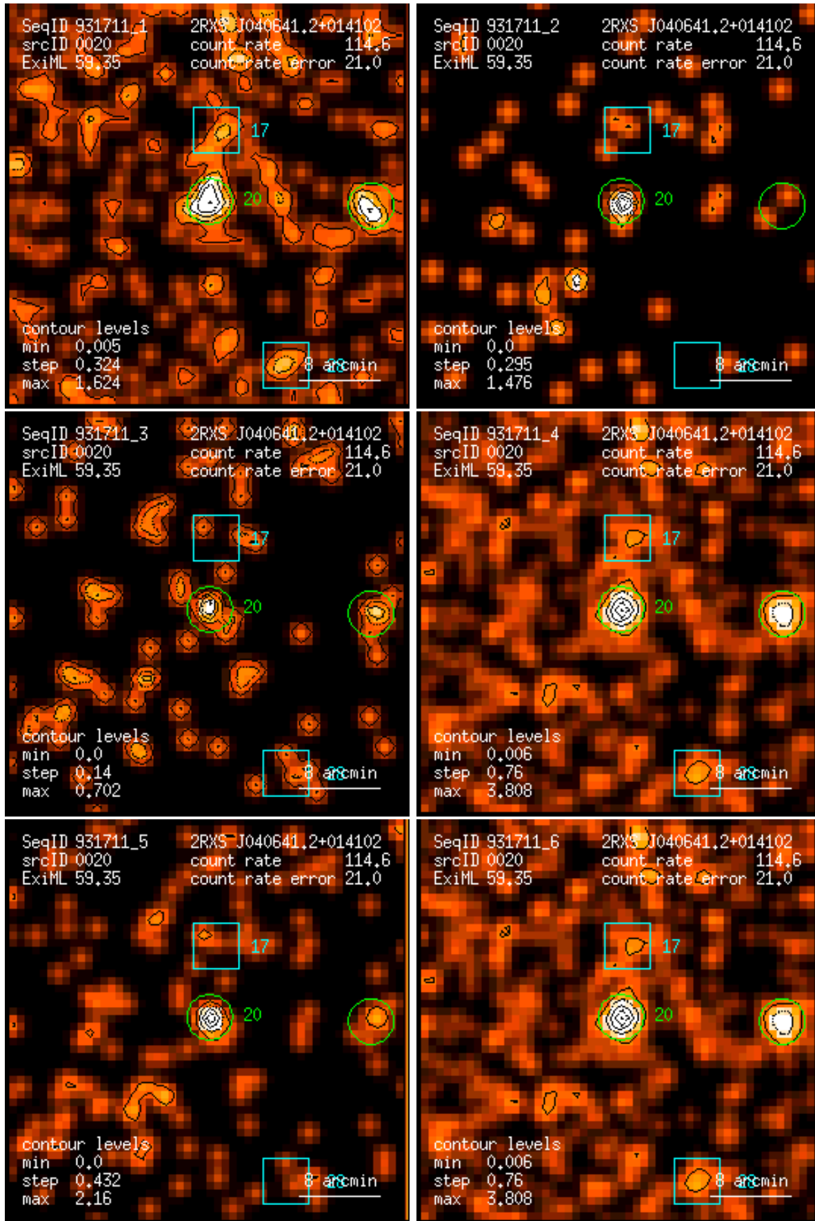
Figure 20: RASS 931711: detection 0020: band rate images, Gaussian filter: (1) PSPC channels 11 – 41, (2) 52 – 90, (3) 91 – 201, (4) 11 – 235, (5) 52 – 201, (6) 11 – 201. Broad band rates in counts/ks. Band rate contour levels in counts/ks/arcmin 2 .
