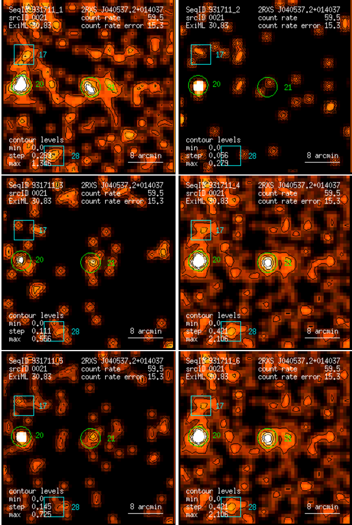
Figure 21: RASS 931711: detection 0021: band rate images, Gaussian filter: (1) PSPC channels 11 – 41, (2) 52 – 90, (3) 91 – 201, (4) 11 – 235, (5) 52 – 201, (6) 11 – 201. Broad band rates in counts/ks. Band rate contour levels in counts/ks/arcmin 2 .
