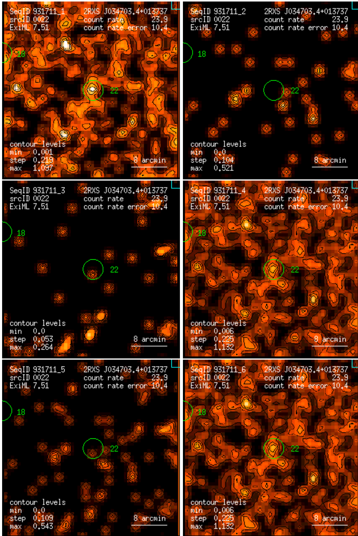
Figure 22: RASS 931711: detection 0022: band rate images, Gaussian filter: (1) PSPC channels 11 – 41, (2) 52 – 90, (3) 91 – 201, (4) 11 – 235, (5) 52 – 201, (6) 11 – 201. Broad band rates in counts/ks. Band rate contour levels in counts/ks/arcmin 2 .
