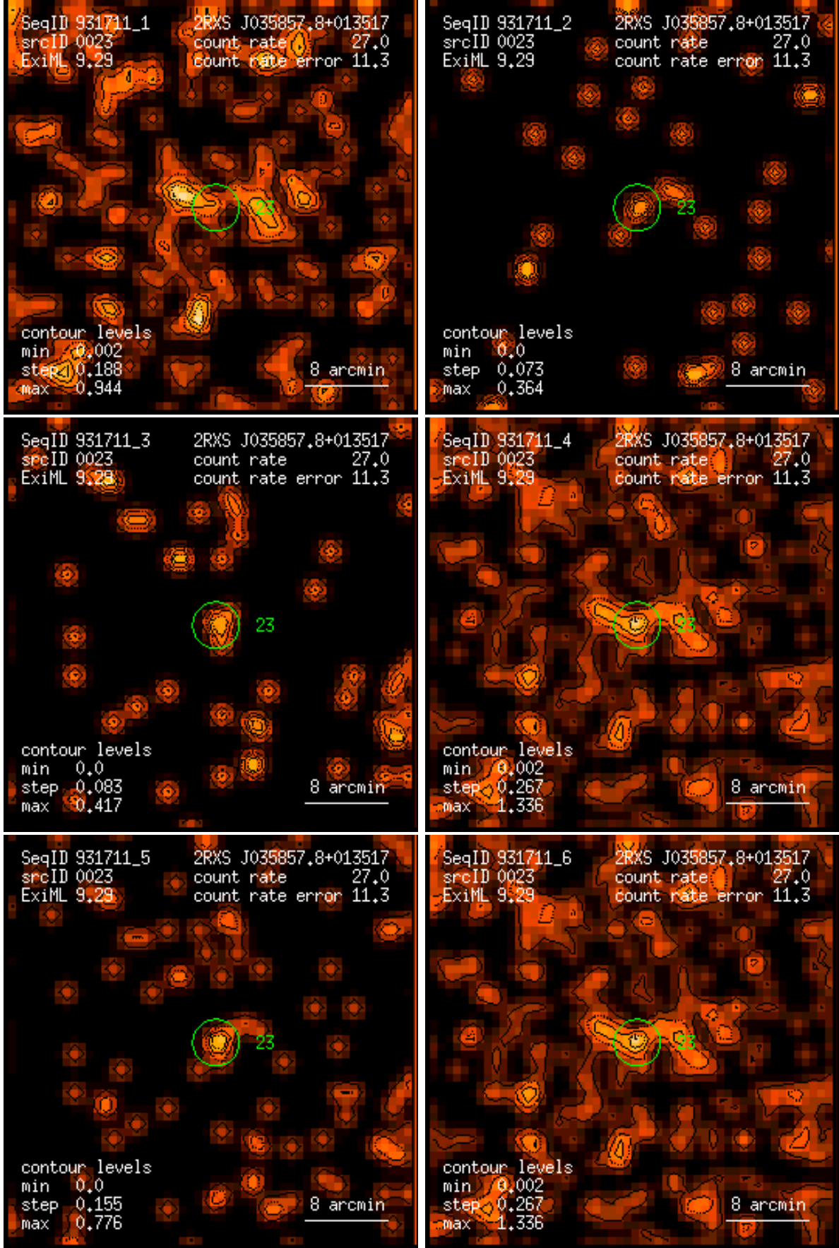
Figure 23: RASS 931711: detection 0023: band rate images, Gaussian filter: (1) PSPC channels 11 – 41, (2) 52 – 90, (3) 91 – 201, (4) 11 – 235, (5) 52 – 201, (6) 11 – 201. Broad band rates in counts/ks. Band rate contour levels in counts/ks/arcmin 2 .
