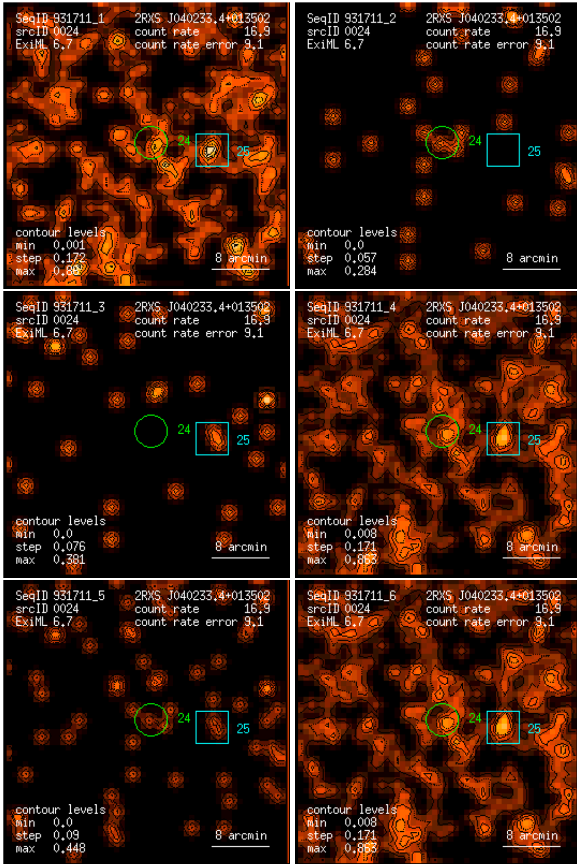
Figure 24: RASS 931711: detection 0024: band rate images, Gaussian filter: (1) PSPC channels 11 – 41, (2) 52 – 90, (3) 91 – 201, (4) 11 – 235, (5) 52 – 201, (6) 11 – 201. Broad band rates in counts/ks. Band rate contour levels in counts/ks/arcmin 2 .
