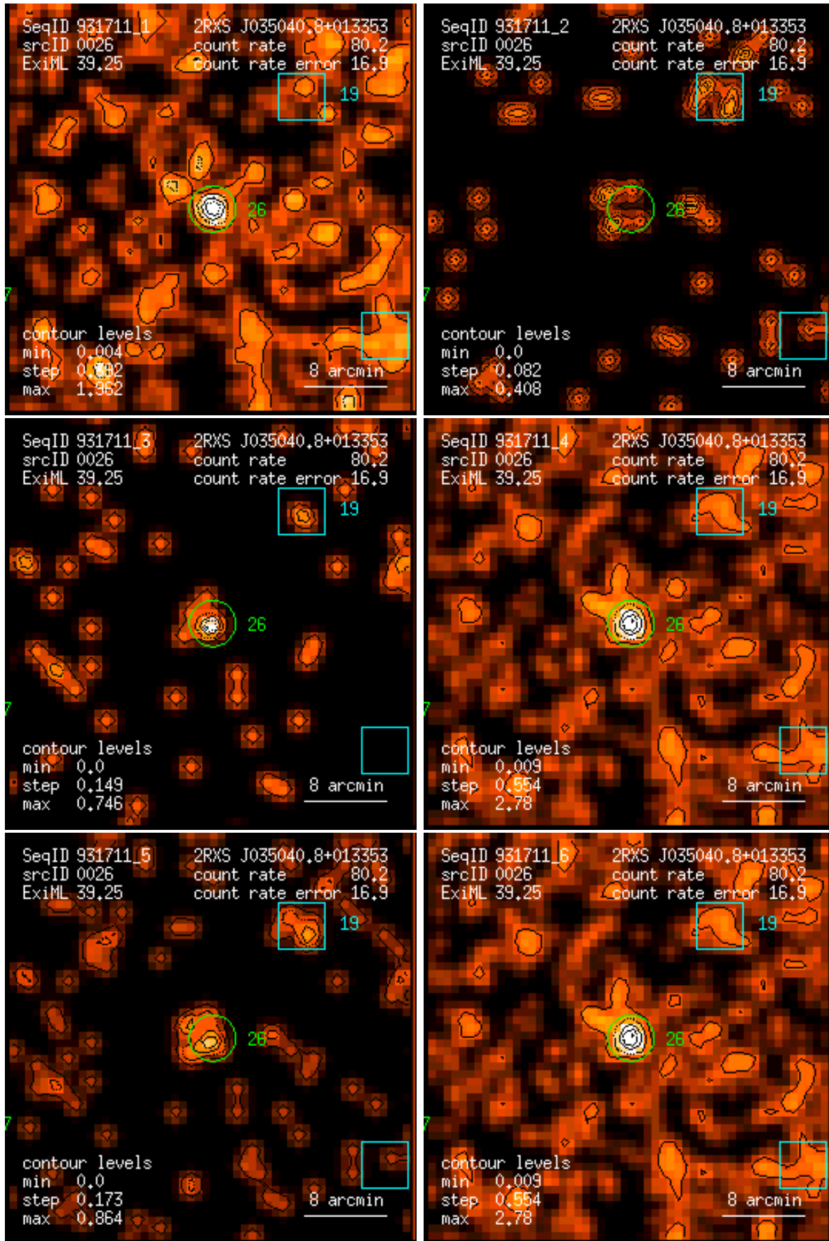
Figure 26: RASS 931711: detection 0026: band rate images, Gaussian filter: (1) PSPC channels 11 – 41, (2) 52 – 90, (3) 91 – 201, (4) 11 – 235, (5) 52 – 201, (6) 11 – 201. Broad band rates in counts/ks. Band rate contour levels in counts/ks/arcmin 2 .
