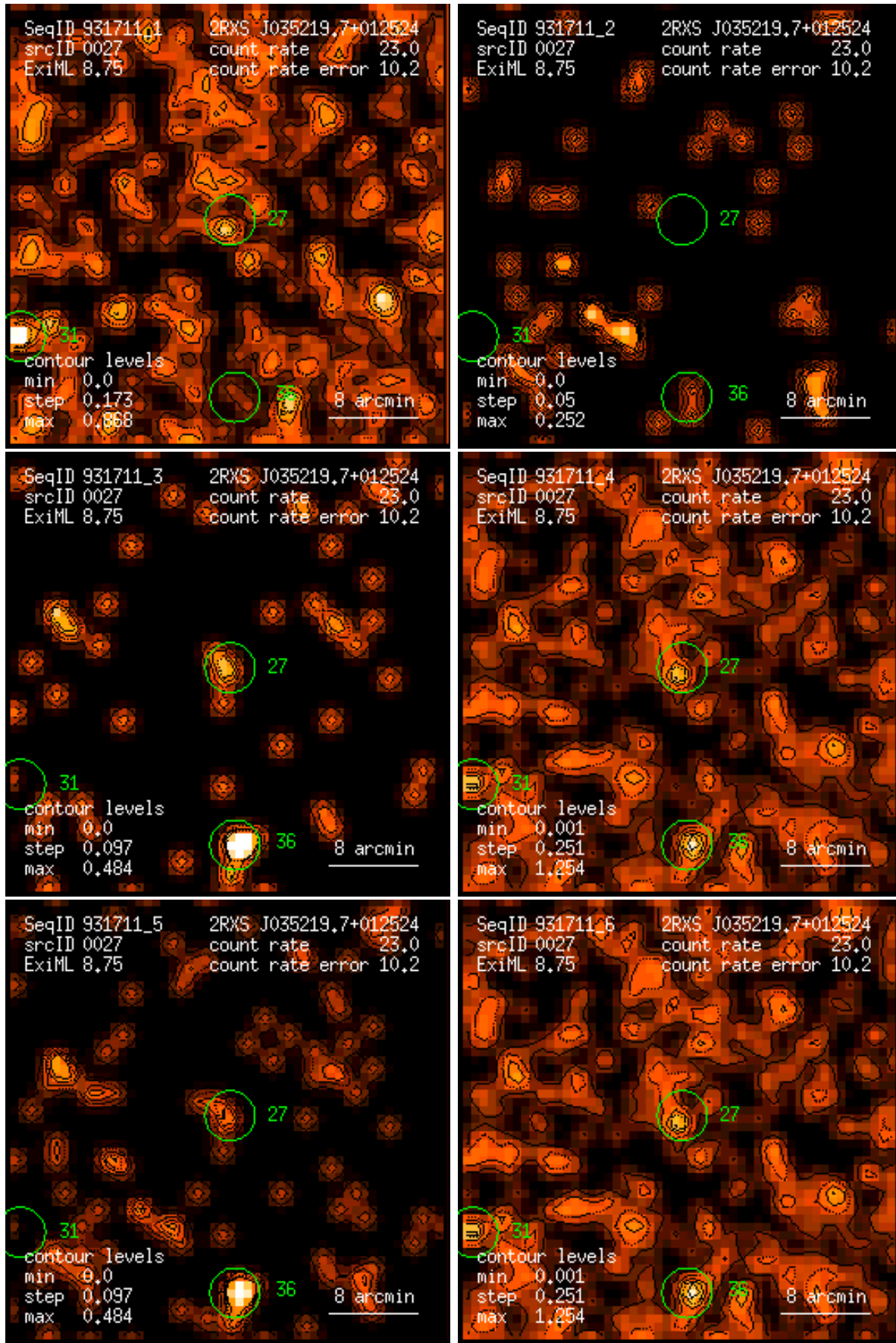
Figure 27: RASS 931711: detection 0027: band rate images, Gaussian filter: (1) PSPC channels 11 – 41, (2) 52 – 90, (3) 91 – 201, (4) 11 – 235, (5) 52 – 201, (6) 11 – 201. Broad band rates in counts/ks. Band rate contour levels in counts/ks/arcmin 2 .
