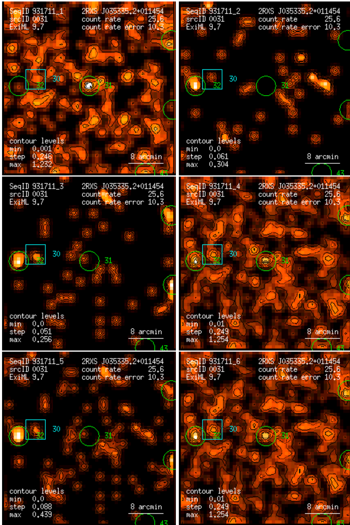
Figure 31: RASS 931711: detection 0031: band rate images, Gaussian filter: (1) PSPC channels 11 – 41, (2) 52 – 90, (3) 91 – 201, (4) 11 – 235, (5) 52 – 201, (6) 11 – 201. Broad band rates in counts/ks. Band rate contour levels in counts/ks/arcmin 2 .
