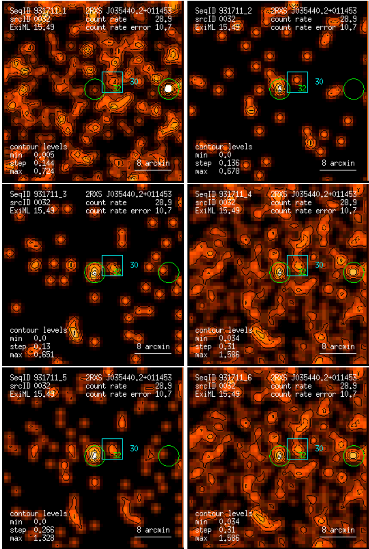
Figure 32: RASS 931711: detection 0032: band rate images, Gaussian filter: (1) PSPC channels 11 – 41, (2) 52 – 90, (3) 91 – 201, (4) 11 – 235, (5) 52 – 201, (6) 11 – 201. Broad band rates in counts/ks. Band rate contour levels in counts/ks/arcmin 2 .
