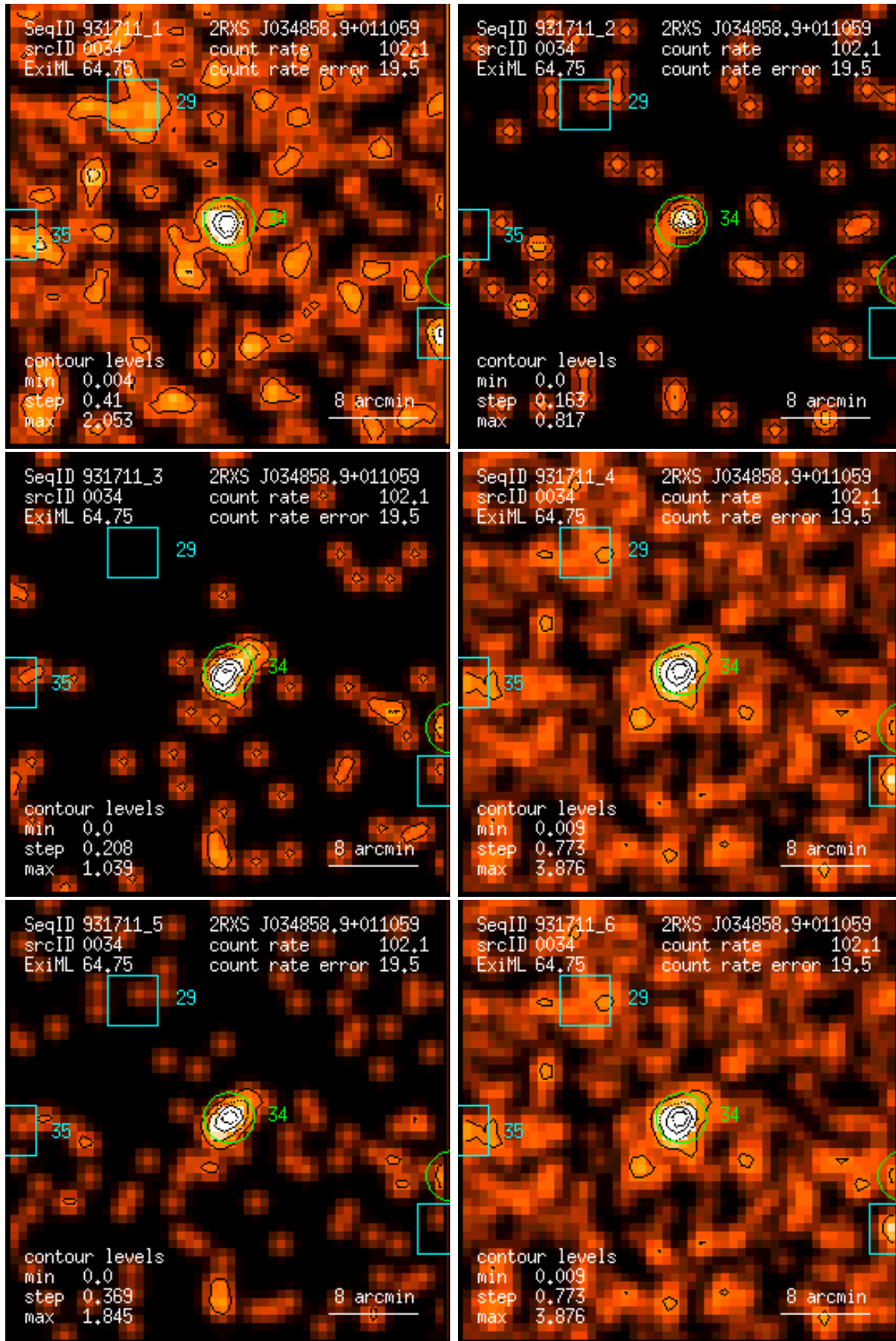
Figure 34: RASS 931711: detection 0034: band rate images, Gaussian filter: (1) PSPC channels 11 – 41, (2) 52 – 90, (3) 91 – 201, (4) 11 – 235, (5) 52 – 201, (6) 11 – 201. Broad band rates in counts/ks. Band rate contour levels in counts/ks/arcmin 2 .
