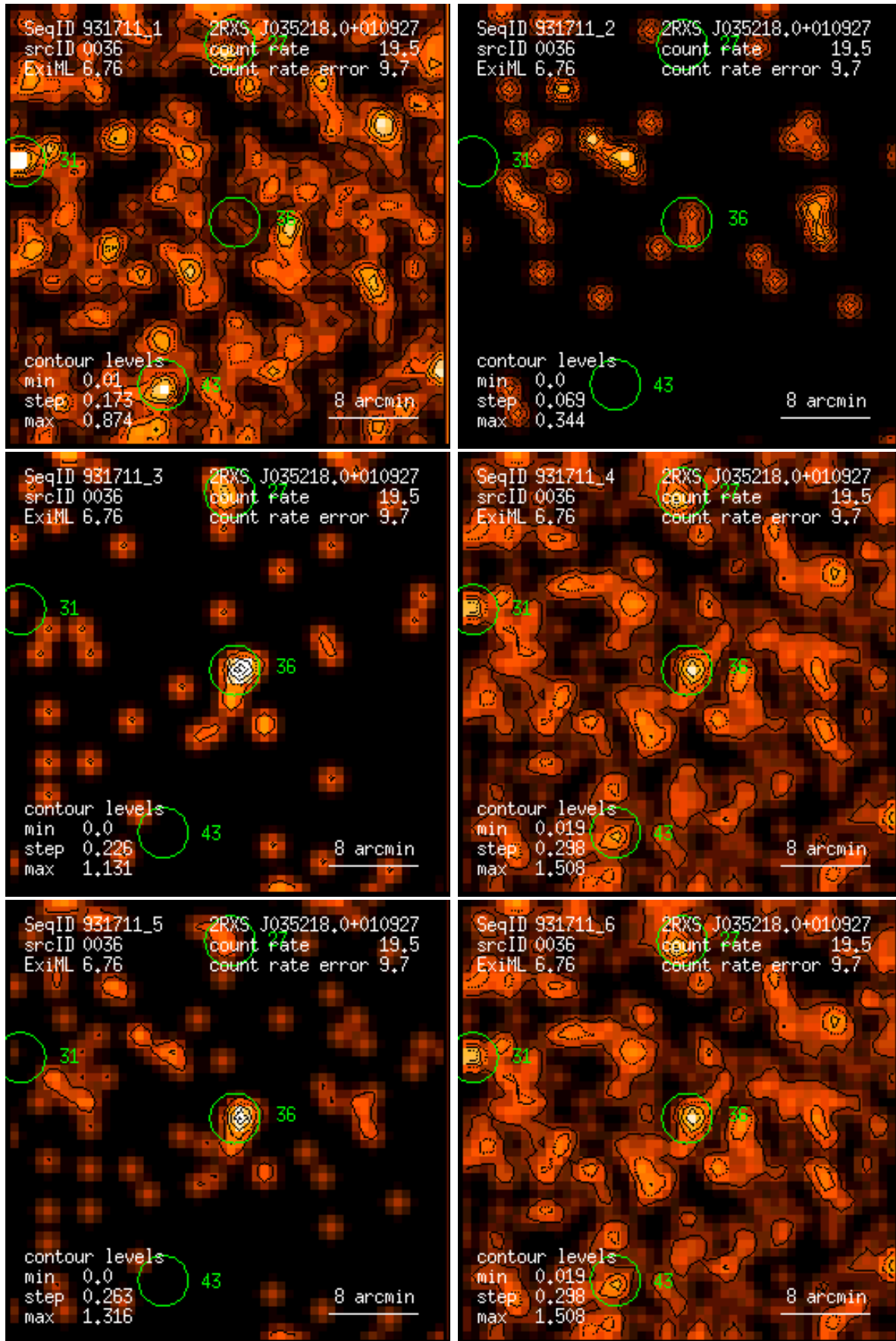
Figure 36: RASS 931711: detection 0036: band rate images, Gaussian filter: (1) PSPC channels 11 – 41, (2) 52 – 90, (3) 91 – 201, (4) 11 – 235, (5) 52 – 201, (6) 11 – 201. Broad band rates in counts/ks. Band rate contour levels in counts/ks/arcmin 2 .
