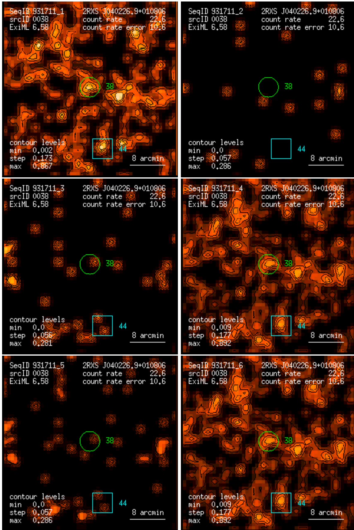
Figure 38: RASS 931711: detection 0038: band rate images, Gaussian filter: (1) PSPC channels 11 – 41, (2) 52 – 90, (3) 91 – 201, (4) 11 – 235, (5) 52 – 201, (6) 11 – 201. Broad band rates in counts/ks. Band rate contour levels in counts/ks/arcmin 2 .
