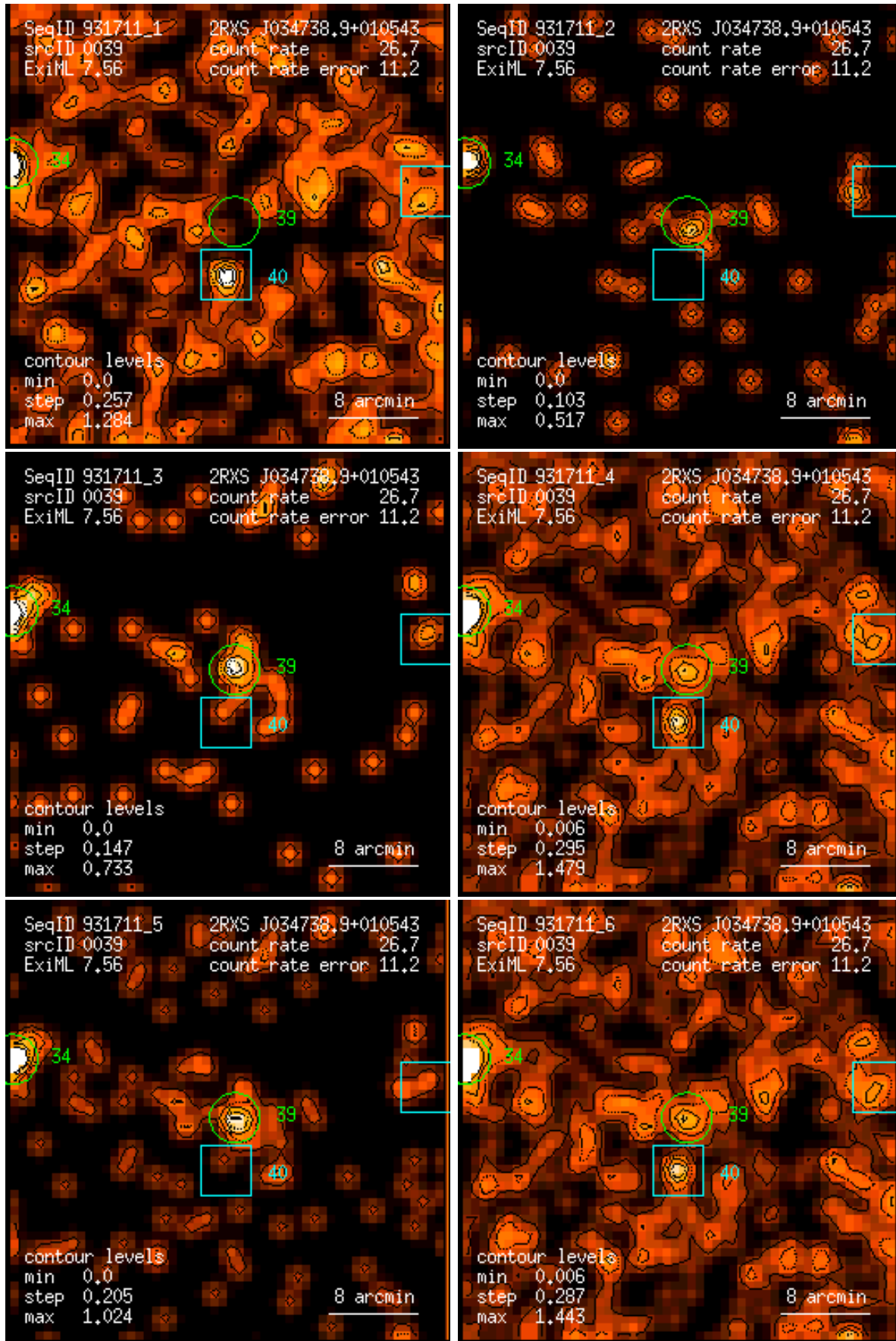
Figure 39: RASS 931711: detection 0039: band rate images, Gaussian filter: (1) PSPC channels 11 – 41, (2) 52 – 90, (3) 91 – 201, (4) 11 – 235, (5) 52 – 201, (6) 11 – 201. Broad band rates in counts/ks. Band rate contour levels in counts/ks/arcmin 2 .
