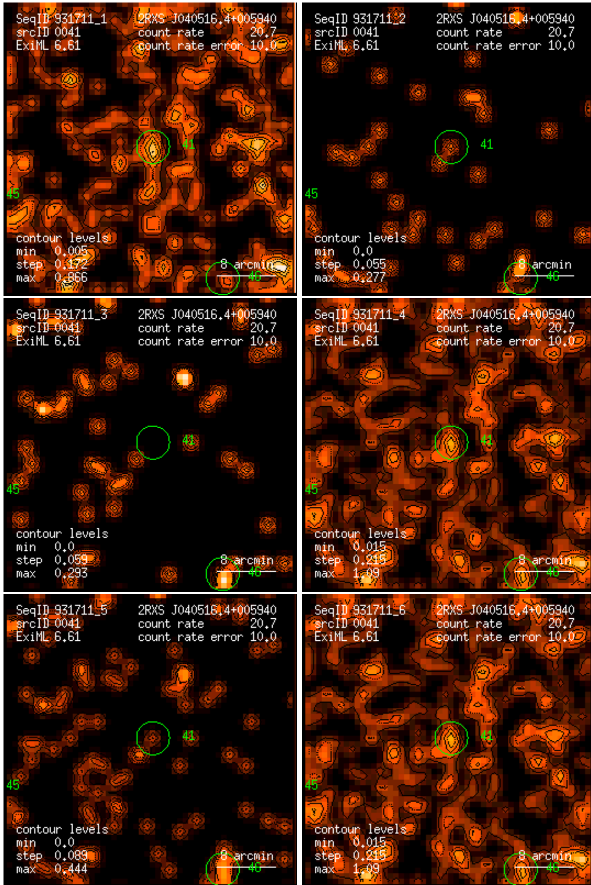
Figure 41: RASS 931711: detection 0041: band rate images, Gaussian filter: (1) PSPC channels 11 – 41, (2) 52 – 90, (3) 91 – 201, (4) 11 – 235, (5) 52 – 201, (6) 11 – 201. Broad band rates in counts/ks. Band rate contour levels in counts/ks/arcmin 2 .
