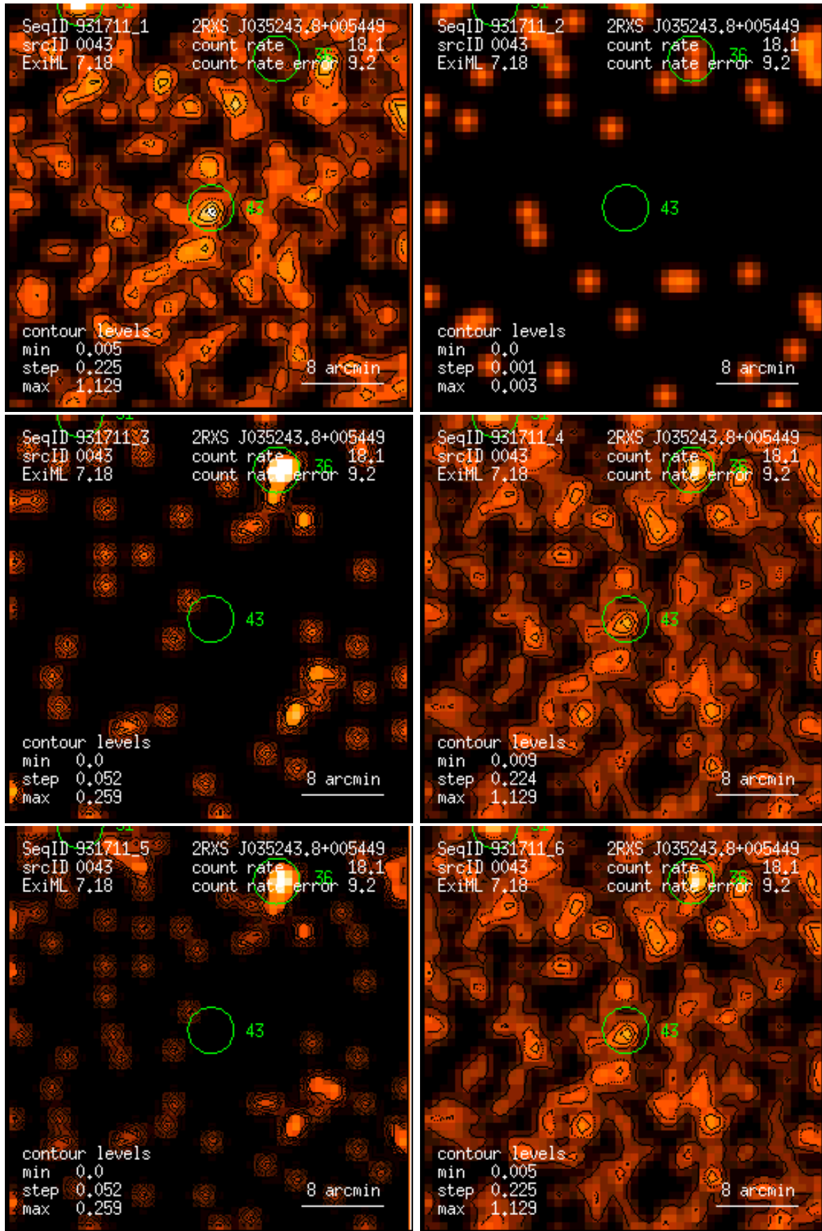
Figure 43: RASS 931711: detection 0043: band rate images, Gaussian filter: (1) PSPC channels 11 – 41, (2) 52 – 90, (3) 91 – 201, (4) 11 – 235, (5) 52 – 201, (6) 11 – 201. Broad band rates in counts/ks. Band rate contour levels in counts/ks/arcmin 2 .
