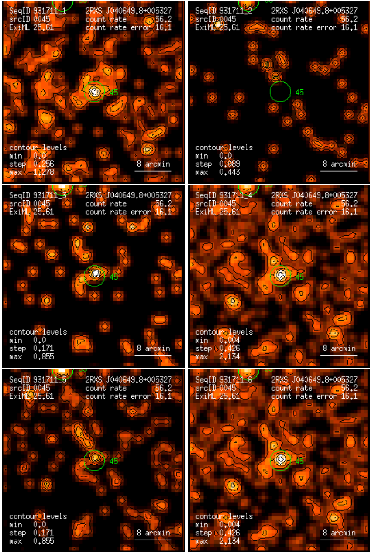
Figure 45: RASS 931711: detection 0045: band rate images, Gaussian filter: (1) PSPC channels 11 – 41, (2) 52 – 90, (3) 91 – 201, (4) 11 – 235, (5) 52 – 201, (6) 11 – 201. Broad band rates in counts/ks. Band rate contour levels in counts/ks/arcmin 2 .
