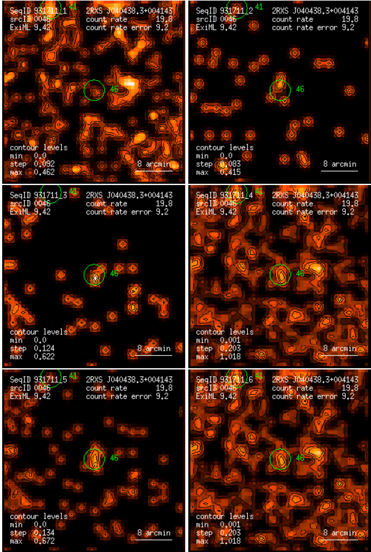
Figure 46: RASS 931711: detection 0046: band rate images, Gaussian filter: (1) PSPC channels 11 – 41, (2) 52 – 90, (3) 91 – 201, (4) 11 – 235, (5) 52 – 201, (6) 11 – 201. Broad band rates in counts/ks. Band rate contour levels in counts/ks/arcmin 2 .
