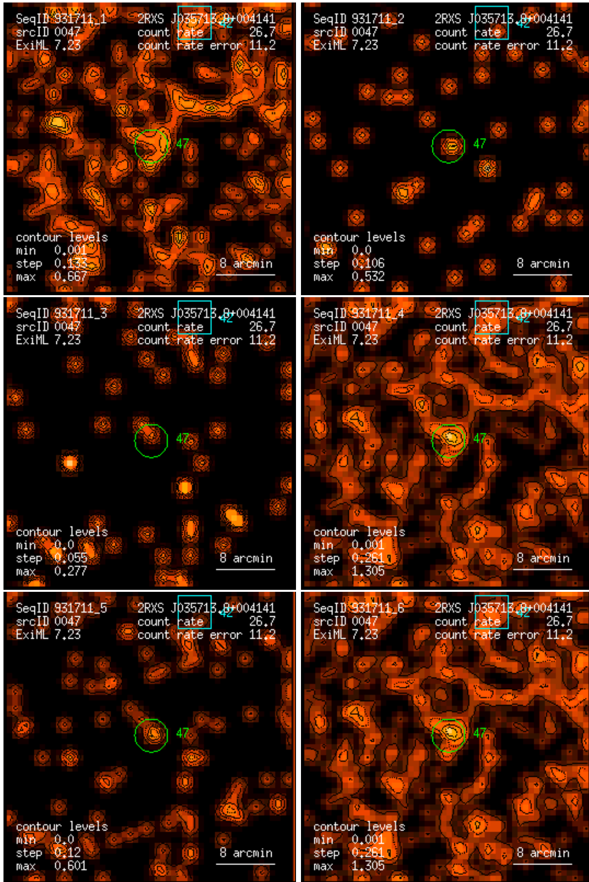
Figure 47: RASS 931711: detection 0047: band rate images, Gaussian filter: (1) PSPC channels 11 – 41, (2) 52 – 90, (3) 91 – 201, (4) 11 – 235, (5) 52 – 201, (6) 11 – 201. Broad band rates in counts/ks. Band rate contour levels in counts/ks/arcmin 2 .
