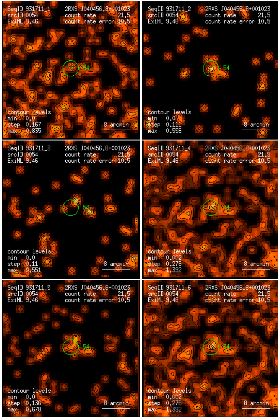
Figure 54: RASS 931711: detection 0054: band rate images, Gaussian filter: (1) PSPC channels 11 – 41, (2) 52 – 90, (3) 91 – 201, (4) 11 – 235, (5) 52 – 201, (6) 11 – 201. Broad band rates in counts/ks. Band rate contour levels in counts/ks/arcmin 2 .
