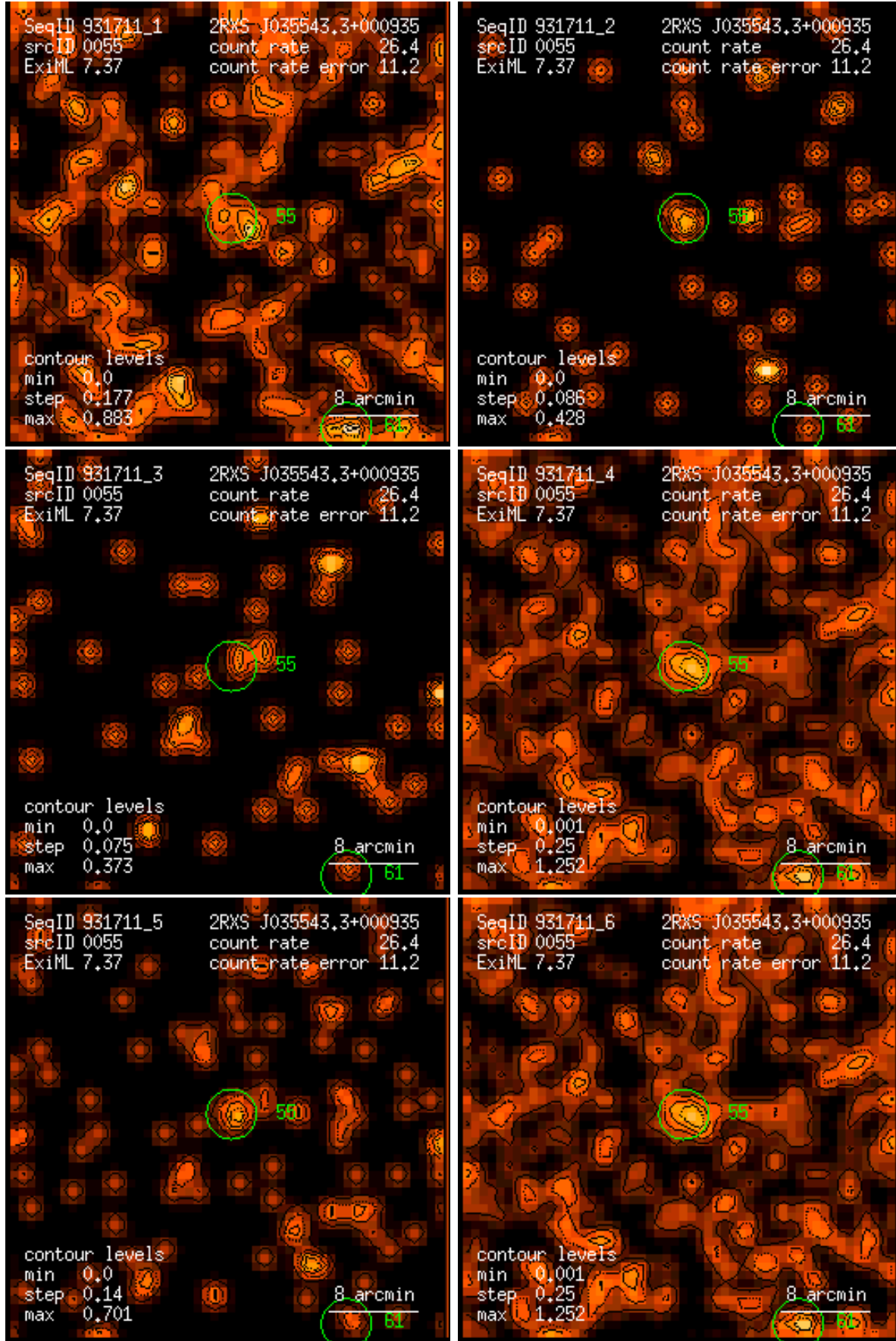
Figure 55: RASS 931711: detection 0055: band rate images, Gaussian filter: (1) PSPC channels 11 – 41, (2) 52 – 90, (3) 91 – 201, (4) 11 – 235, (5) 52 – 201, (6) 11 – 201. Broad band rates in counts/ks. Band rate contour levels in counts/ks/arcmin 2 .
