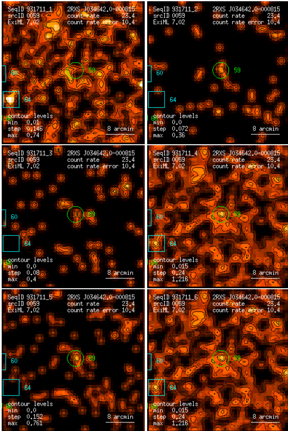
Figure 59: RASS 931711: detection 0059: band rate images, Gaussian filter: (1) PSPC channels 11 – 41, (2) 52 – 90, (3) 91 – 201, (4) 11 – 235, (5) 52 – 201, (6) 11 – 201. Broad band rates in counts/ks. Band rate contour levels in counts/ks/arcmin 2 .
