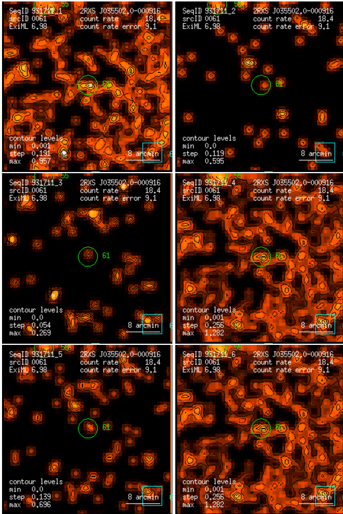
Figure 61: RASS 931711: detection 0061: band rate images, Gaussian filter: (1) PSPC channels 11 – 41, (2) 52 – 90, (3) 91 – 201, (4) 11 – 235, (5) 52 – 201, (6) 11 – 201. Broad band rates in counts/ks. Band rate contour levels in counts/ks/arcmin 2 .
