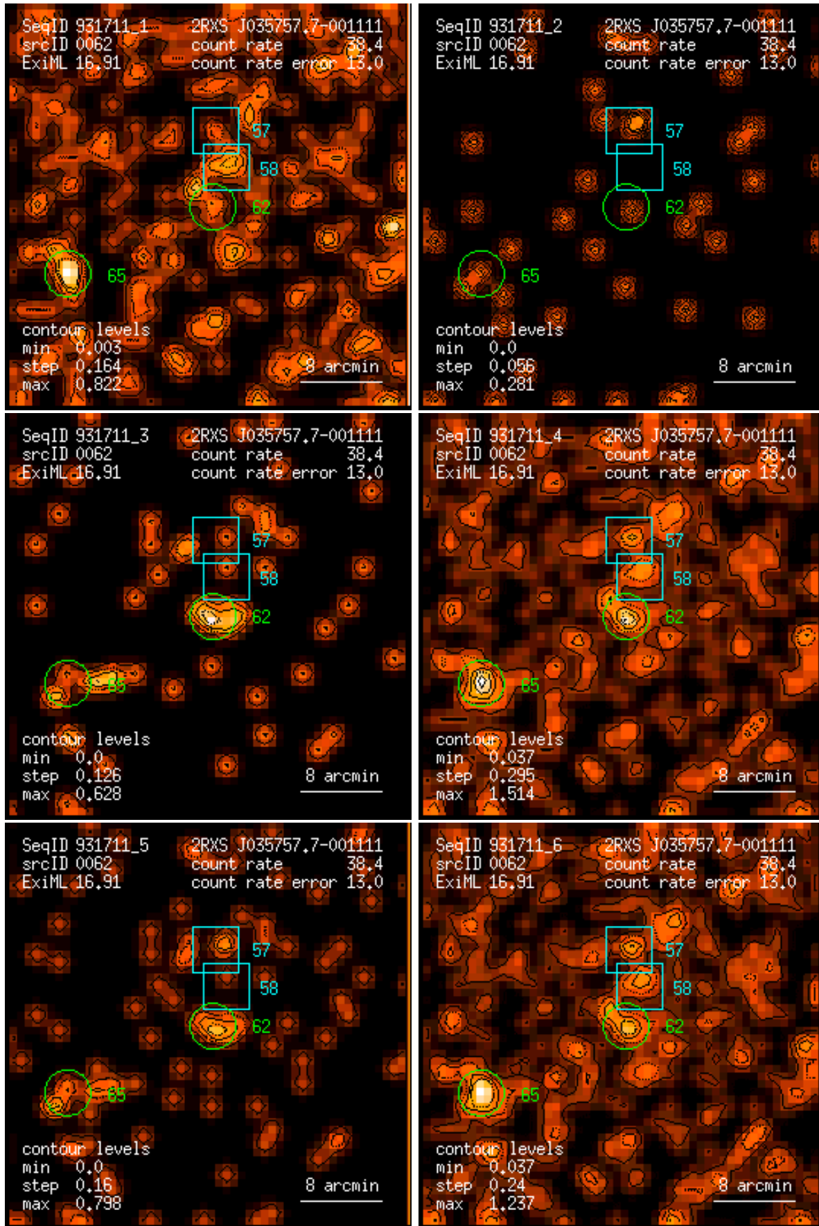
Figure 62: RASS 931711: detection 0062: band rate images, Gaussian filter: (1) PSPC channels 11 – 41, (2) 52 – 90, (3) 91 – 201, (4) 11 – 235, (5) 52 – 201, (6) 11 – 201. Broad band rates in counts/ks. Band rate contour levels in counts/ks/arcmin 2 .
