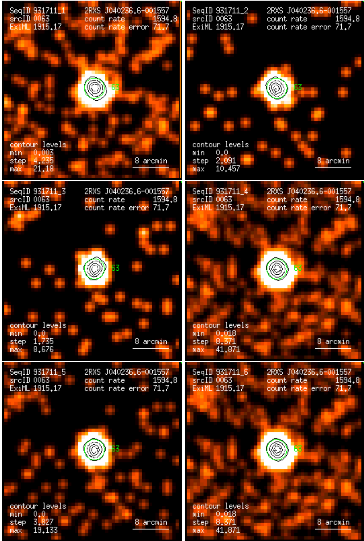
Figure 63: RASS 931711: detection 0063: band rate images, Gaussian filter: (1) PSPC channels 11 – 41, (2) 52 – 90, (3) 91 – 201, (4) 11 – 235, (5) 52 – 201, (6) 11 – 201. Broad band rates in counts/ks. Band rate contour levels in counts/ks/arcmin 2 .
