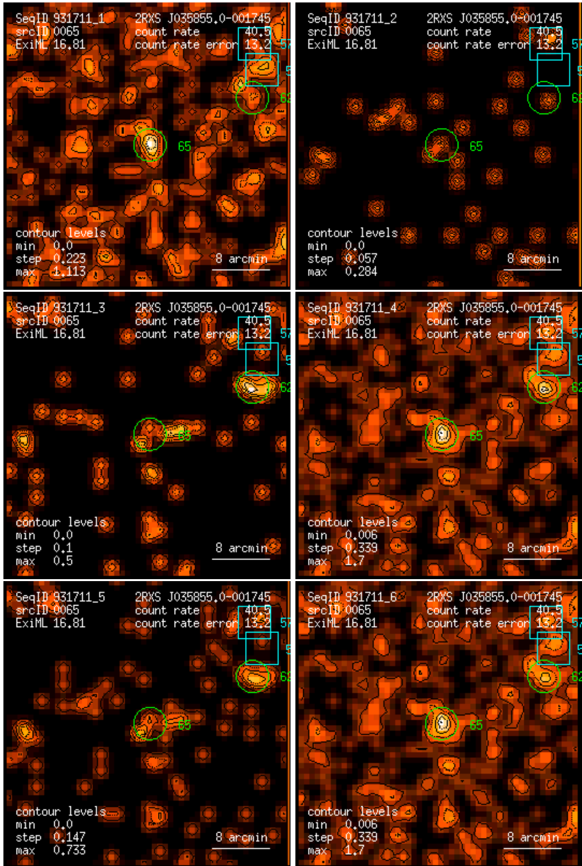
Figure 65: RASS 931711: detection 0065: band rate images, Gaussian filter: (1) PSPC channels 11 – 41, (2) 52 – 90, (3) 91 – 201, (4) 11 – 235, (5) 52 – 201, (6) 11 – 201. Broad band rates in counts/ks. Band rate contour levels in counts/ks/arcmin 2 .
