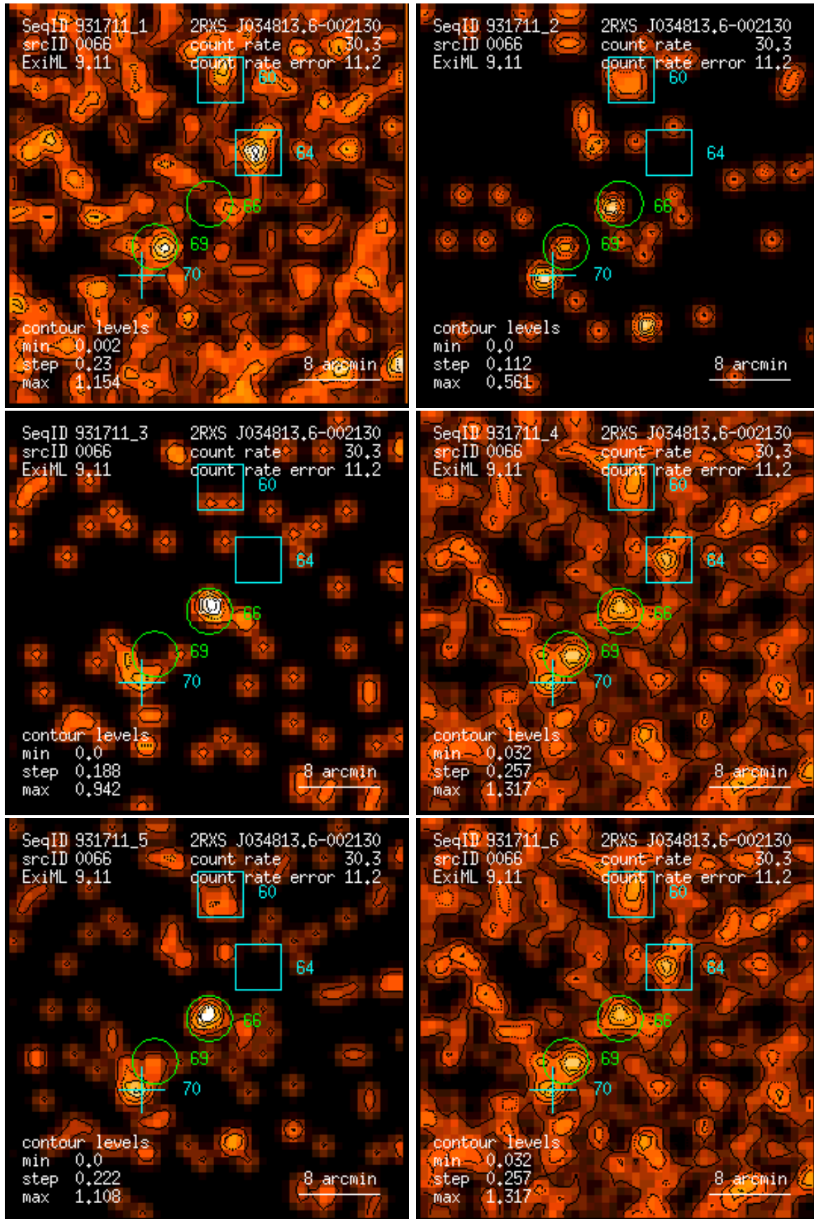
Figure 66: RASS 931711: detection 0066: band rate images, Gaussian filter: (1) PSPC channels 11 – 41, (2) 52 – 90, (3) 91 – 201, (4) 11 – 235, (5) 52 – 201, (6) 11 – 201. Broad band rates in counts/ks. Band rate contour levels in counts/ks/arcmin 2 .
