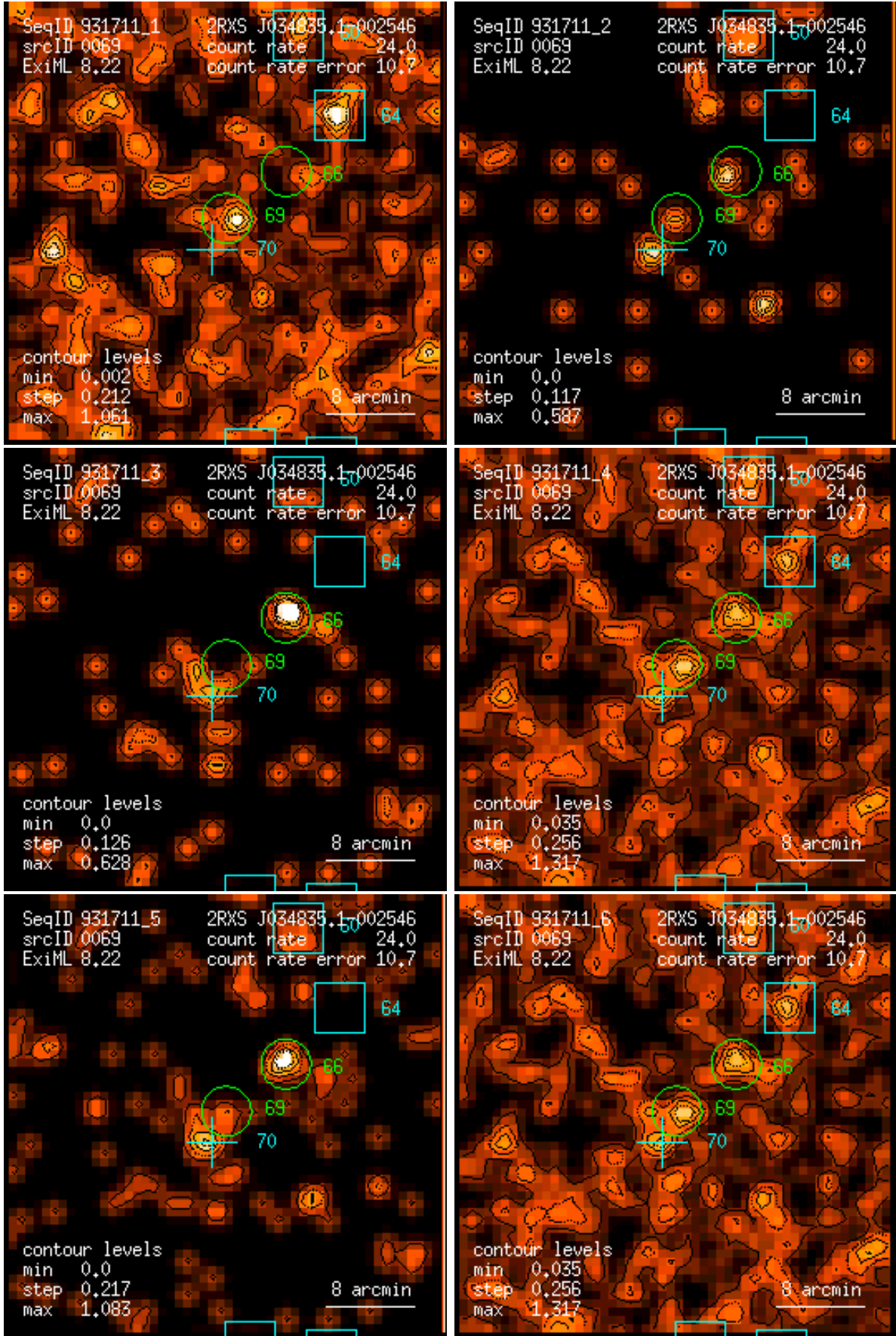
Figure 69: RASS 931711: detection 0069: band rate images, Gaussian filter: (1) PSPC channels 11 – 41, (2) 52 – 90, (3) 91 – 201, (4) 11 – 235, (5) 52 – 201, (6) 11 – 201. Broad band rates in counts/ks. Band rate contour levels in counts/ks/arcmin 2 .
