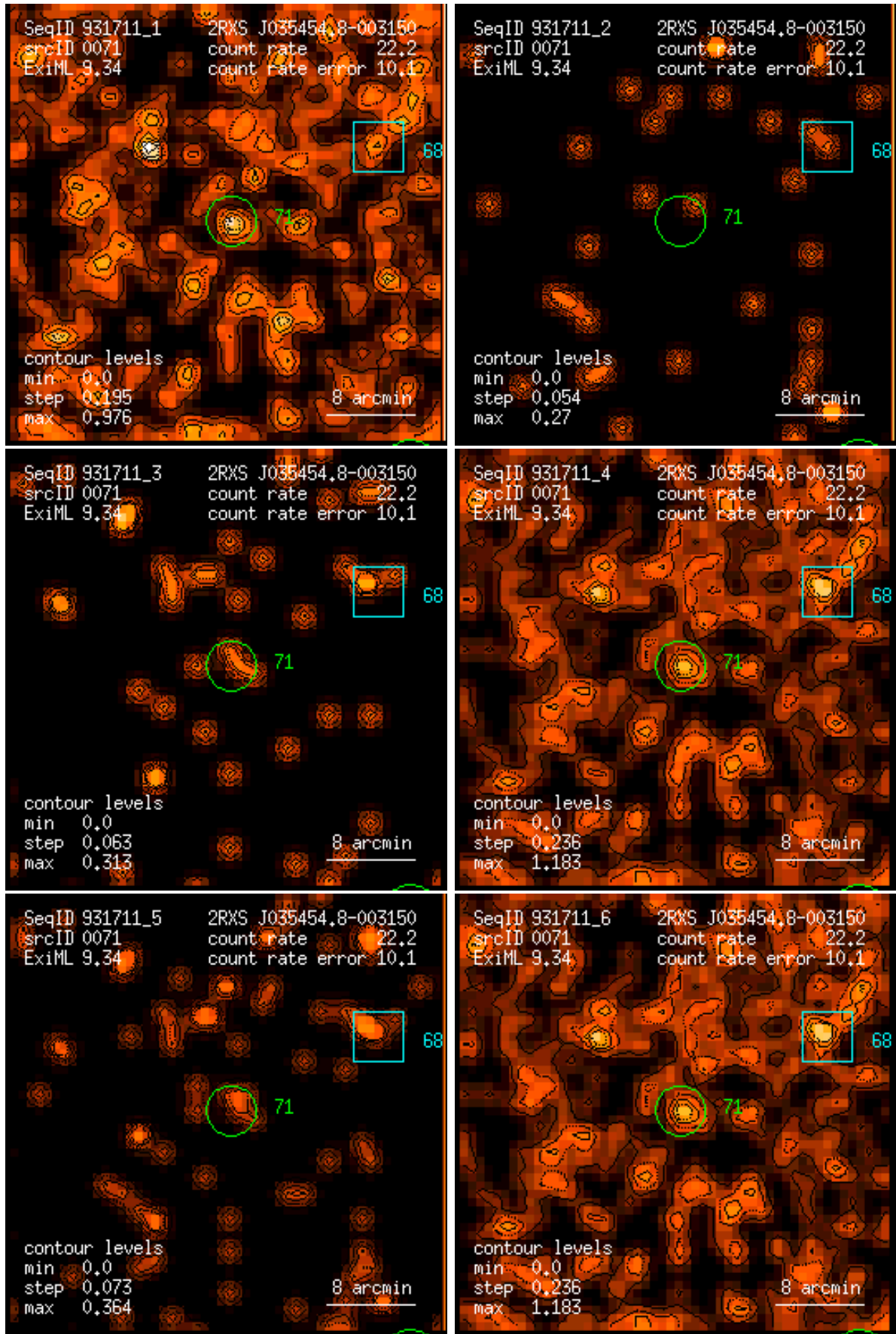
Figure 71: RASS 931711: detection 0071: band rate images, Gaussian filter: (1) PSPC channels 11 – 41, (2) 52 – 90, (3) 91 – 201, (4) 11 – 235, (5) 52 – 201, (6) 11 – 201. Broad band rates in counts/ks. Band rate contour levels in counts/ks/arcmin 2 .
