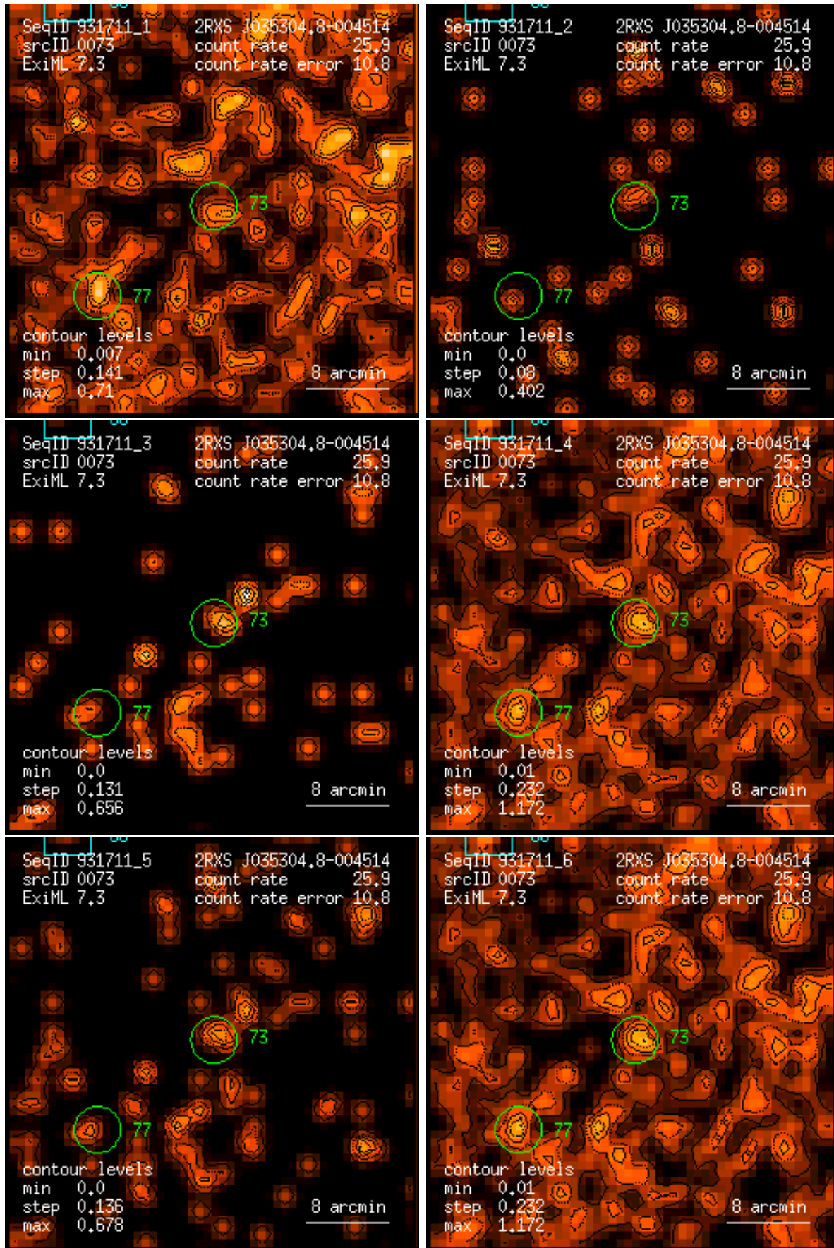
Figure 73: RASS 931711: detection 0073: band rate images, Gaussian filter: (1) PSPC channels 11 – 41, (2) 52 – 90, (3) 91 – 201, (4) 11 – 235, (5) 52 – 201, (6) 11 – 201. Broad band rates in counts/ks. Band rate contour levels in counts/ks/arcmin 2 .
