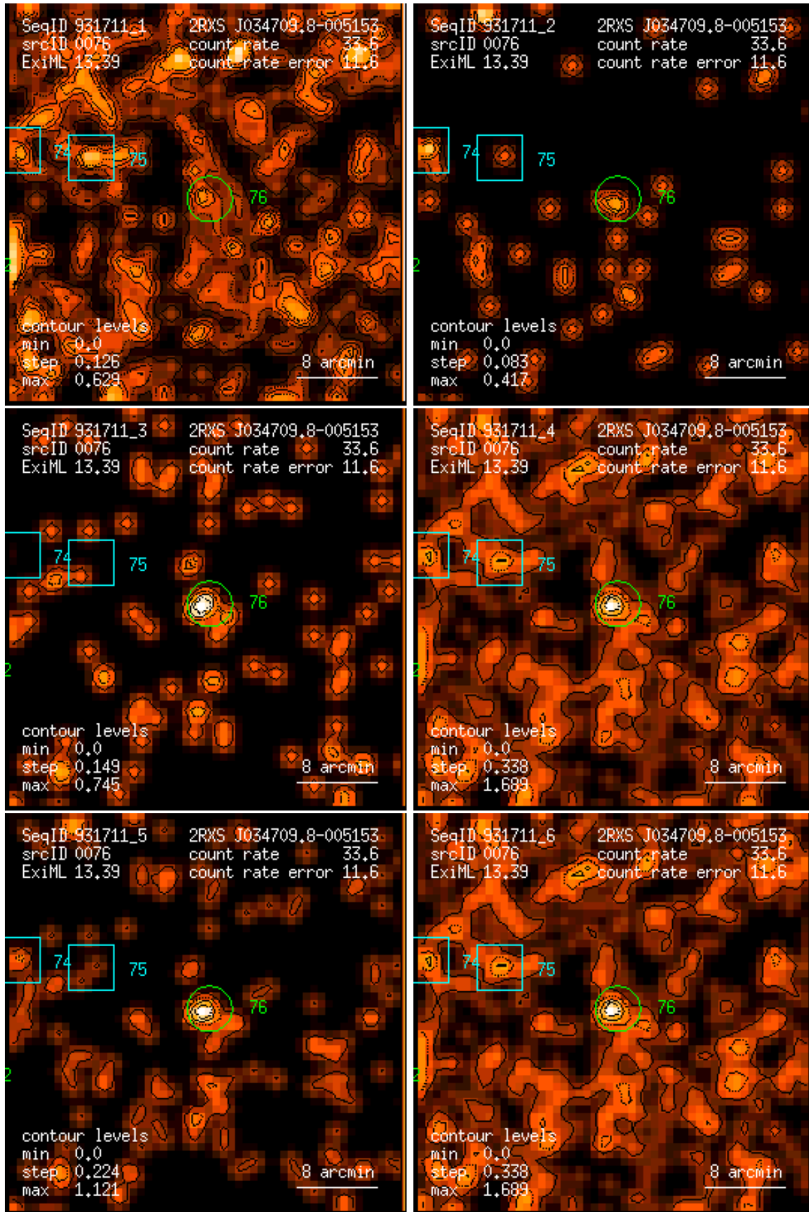
Figure 76: RASS 931711: detection 0076: band rate images, Gaussian filter: (1) PSPC channels 11 – 41, (2) 52 – 90, (3) 91 – 201, (4) 11 – 235, (5) 52 – 201, (6) 11 – 201. Broad band rates in counts/ks. Band rate contour levels in counts/ks/arcmin 2 .
