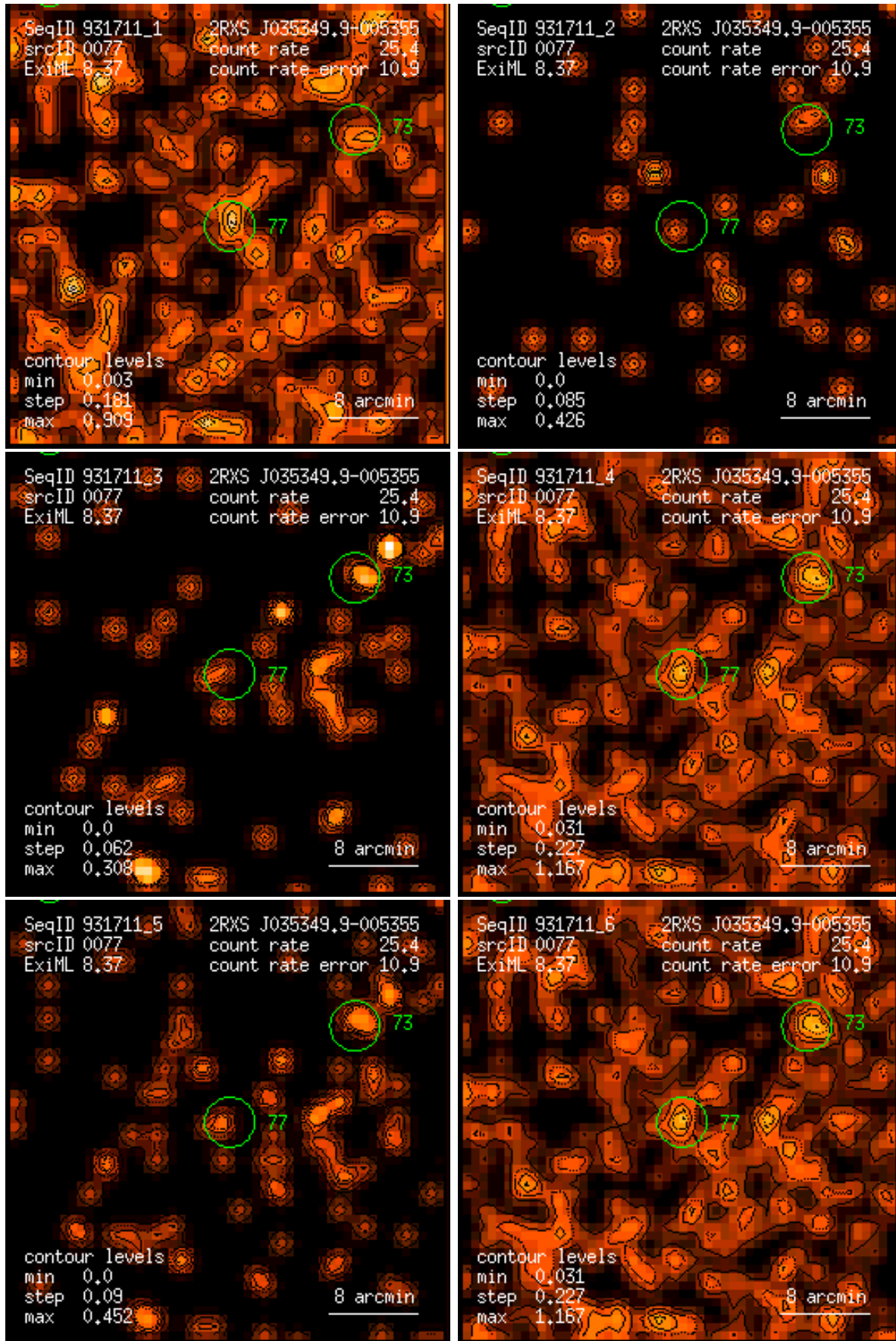
Figure 77: RASS 931711: detection 0077: band rate images, Gaussian filter: (1) PSPC channels 11 – 41, (2) 52 – 90, (3) 91 – 201, (4) 11 – 235, (5) 52 – 201, (6) 11 – 201. Broad band rates in counts/ks. Band rate contour levels in counts/ks/arcmin 2 .
