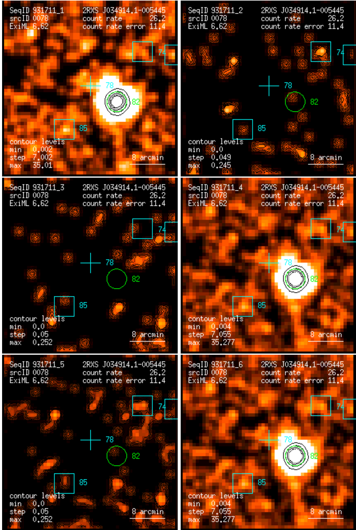
Figure 78: RASS 931711: detection 0078: band rate images, Gaussian filter: (1) PSPC channels 11 – 41, (2) 52 – 90, (3) 91 – 201, (4) 11 – 235, (5) 52 – 201, (6) 11 – 201. Broad band rates in counts/ks. Band rate contour levels in counts/ks/arcmin 2 .
