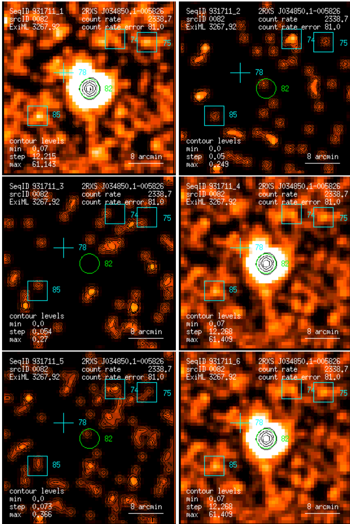
Figure 82: RASS 931711: detection 0082: band rate images, Gaussian filter: (1) PSPC channels 11 – 41, (2) 52 – 90, (3) 91 – 201, (4) 11 – 235, (5) 52 – 201, (6) 11 – 201. Broad band rates in counts/ks. Band rate contour levels in counts/ks/arcmin 2 .
