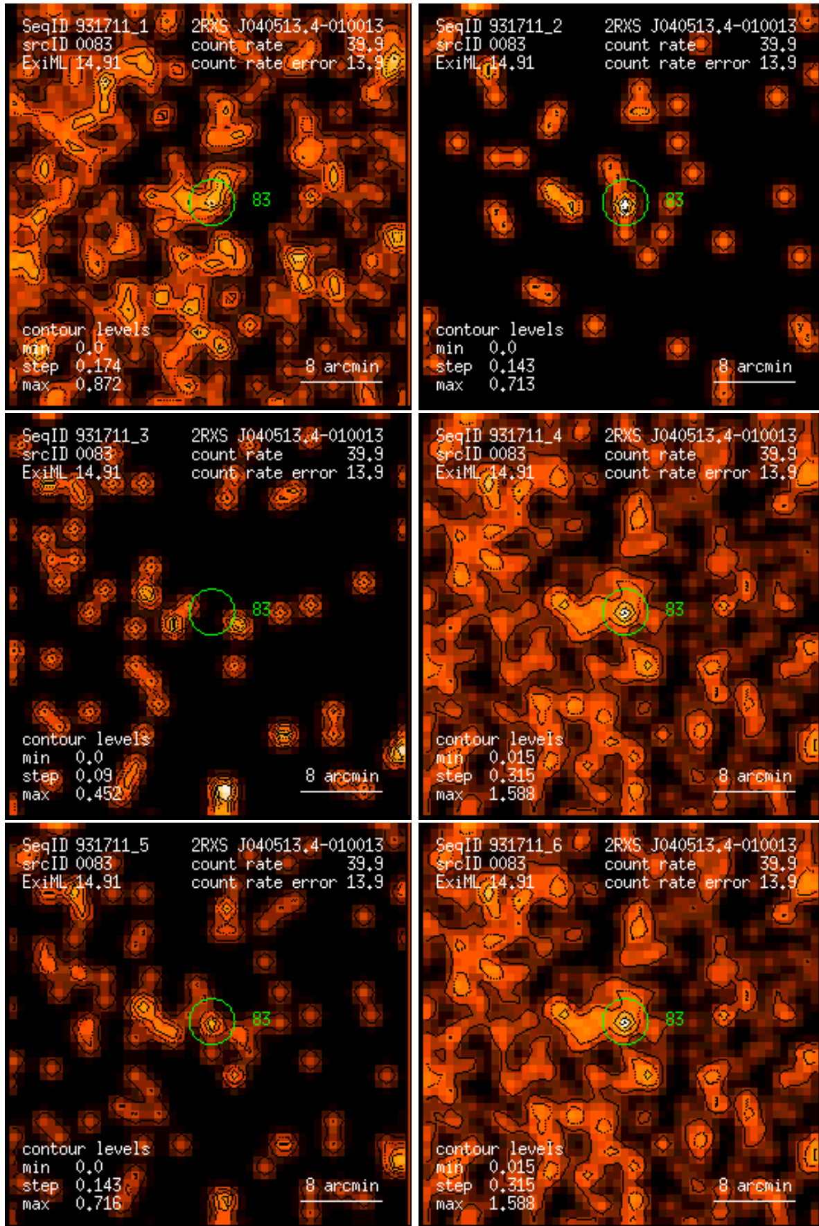
Figure 83: RASS 931711: detection 0083: band rate images, Gaussian filter: (1) PSPC channels 11 – 41, (2) 52 – 90, (3) 91 – 201, (4) 11 – 235, (5) 52 – 201, (6) 11 – 201. Broad band rates in counts/ks. Band rate contour levels in counts/ks/arcmin 2 .
