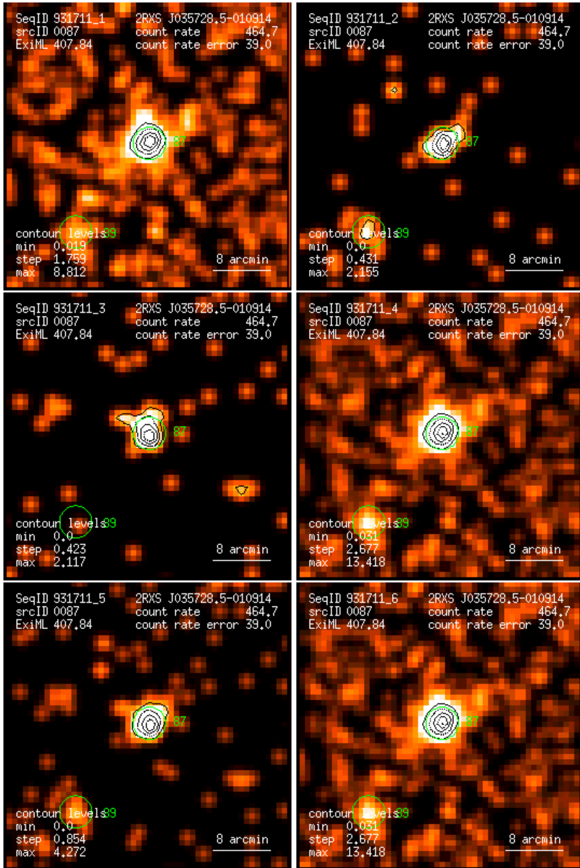
Figure 87: RASS 931711: detection 0087: band rate images, Gaussian filter: (1) PSPC channels 11 – 41, (2) 52 – 90, (3) 91 – 201, (4) 11 – 235, (5) 52 – 201, (6) 11 – 201. Broad band rates in counts/ks. Band rate contour levels in counts/ks/arcmin 2 .
