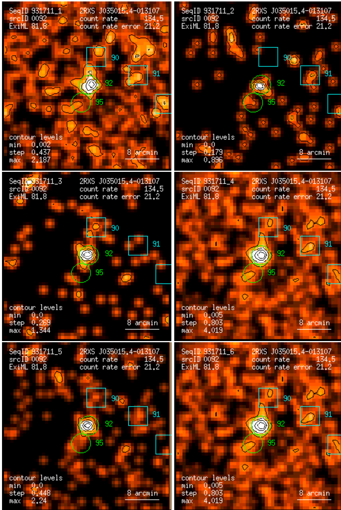
Figure 92: RASS 931711: detection 0092: band rate images, Gaussian filter: (1) PSPC channels 11 – 41, (2) 52 – 90, (3) 91 – 201, (4) 11 – 235, (5) 52 – 201, (6) 11 – 201. Broad band rates in counts/ks. Band rate contour levels in counts/ks/arcmin 2 .
