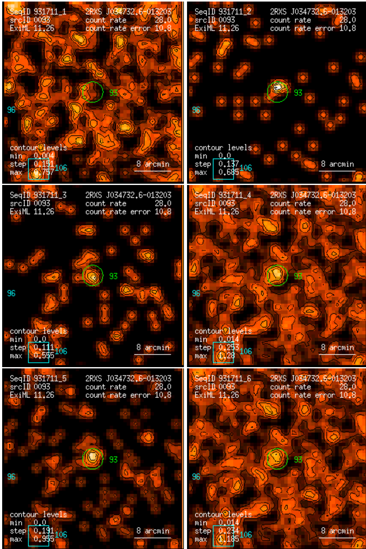
Figure 93: RASS 931711: detection 0093: band rate images, Gaussian filter: (1) PSPC channels 11 – 41, (2) 52 – 90, (3) 91 – 201, (4) 11 – 235, (5) 52 – 201, (6) 11 – 201. Broad band rates in counts/ks. Band rate contour levels in counts/ks/arcmin 2 .
