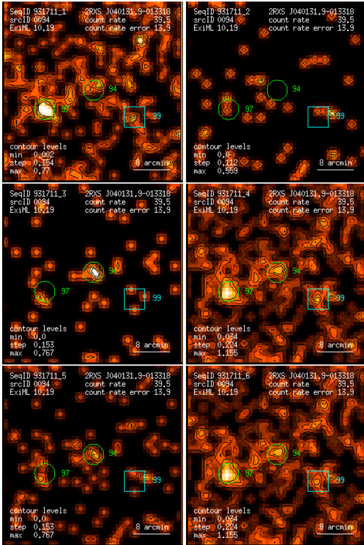
Figure 94: RASS 931711: detection 0094: band rate images, Gaussian filter: (1) PSPC channels 11 – 41, (2) 52 – 90, (3) 91 – 201, (4) 11 – 235, (5) 52 – 201, (6) 11 – 201. Broad band rates in counts/ks. Band rate contour levels in counts/ks/arcmin 2 .
