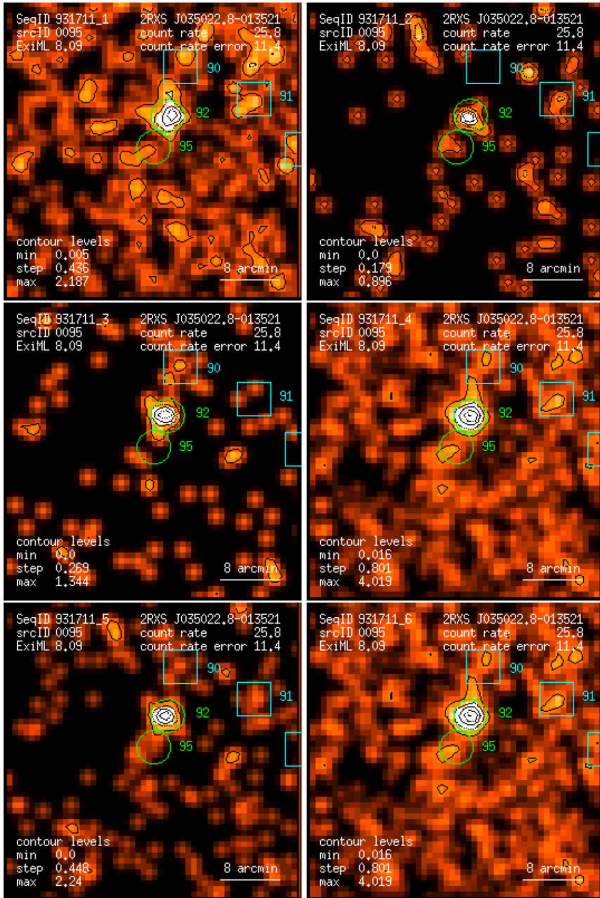
Figure 95: RASS 931711: detection 0095: band rate images, Gaussian filter: (1) PSPC channels 11 – 41, (2) 52 – 90, (3) 91 – 201, (4) 11 – 235, (5) 52 – 201, (6) 11 – 201. Broad band rates in counts/ks. Band rate contour levels in counts/ks/arcmin 2 .
