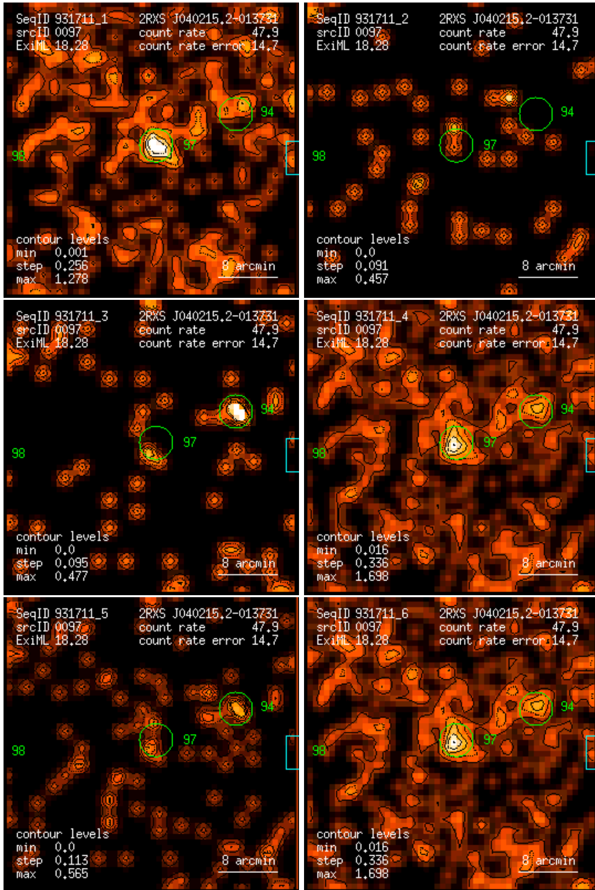
Figure 97: RASS 931711: detection 0097: band rate images, Gaussian filter: (1) PSPC channels 11 – 41, (2) 52 – 90, (3) 91 – 201, (4) 11 – 235, (5) 52 – 201, (6) 11 – 201. Broad band rates in counts/ks. Band rate contour levels in counts/ks/arcmin 2 .
