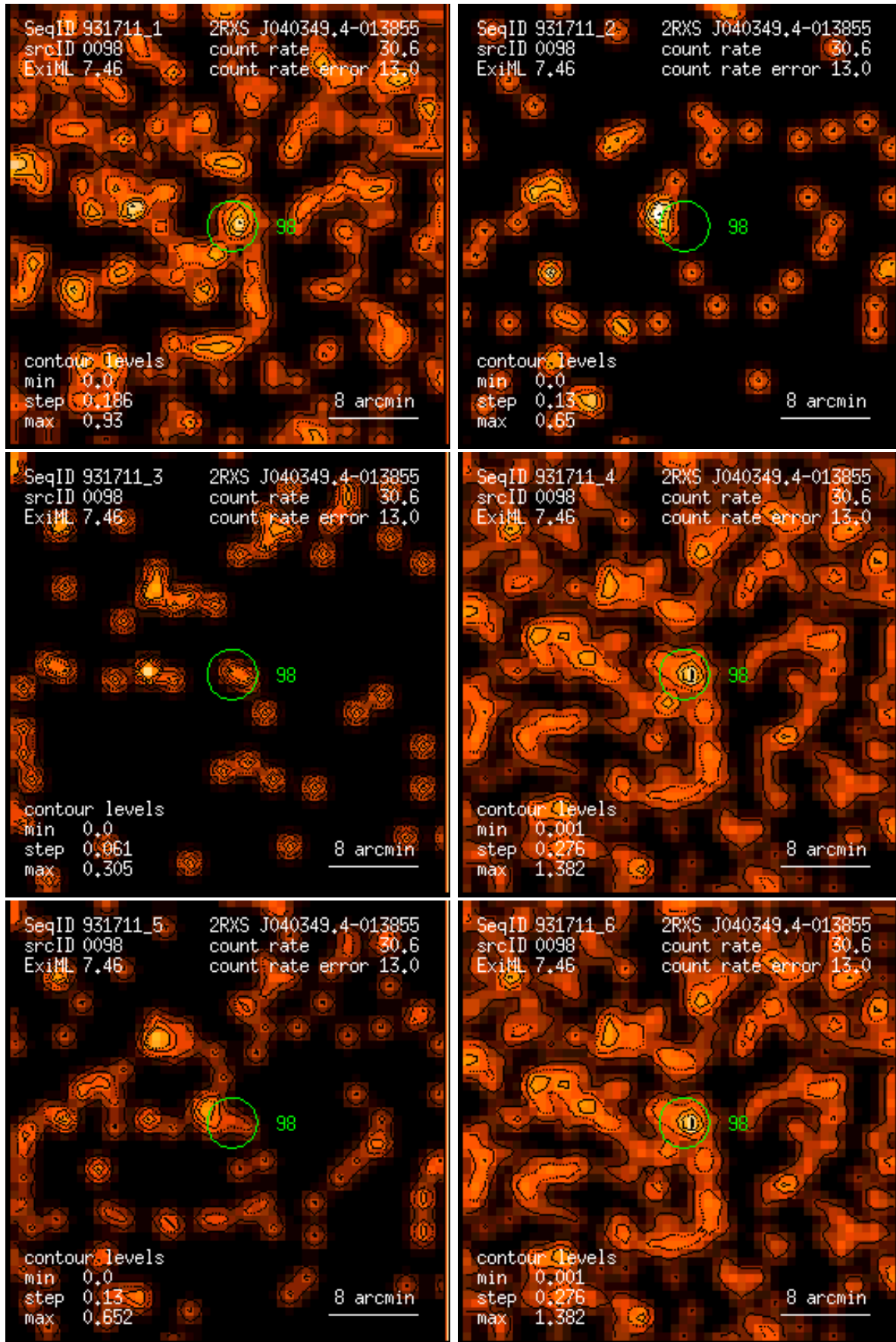
Figure 98: RASS 931711: detection 0098: band rate images, Gaussian filter: (1) PSPC channels 11 – 41, (2) 52 – 90, (3) 91 – 201, (4) 11 – 235, (5) 52 – 201, (6) 11 – 201. Broad band rates in counts/ks. Band rate contour levels in counts/ks/arcmin 2 .
