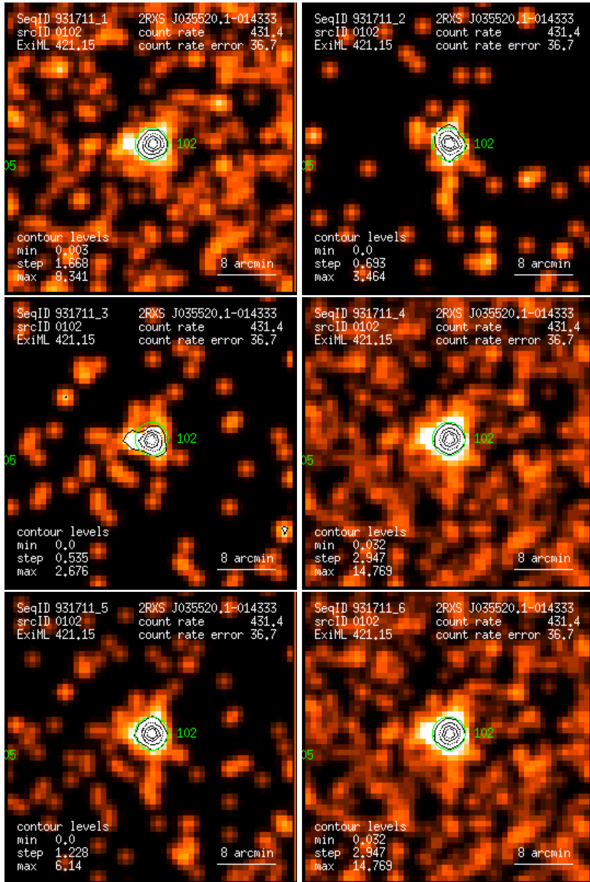
Figure 102: RASS 931711: detection 0102: band rate images, Gaussian filter: (1) PSPC channels 11 – 41, (2) 52 – 90, (3) 91 – 201, (4) 11 – 235, (5) 52 – 201, (6) 11 – 201. Broad band rates in counts/ks. Band rate contour levels in counts/ks/arcmin 2 .
