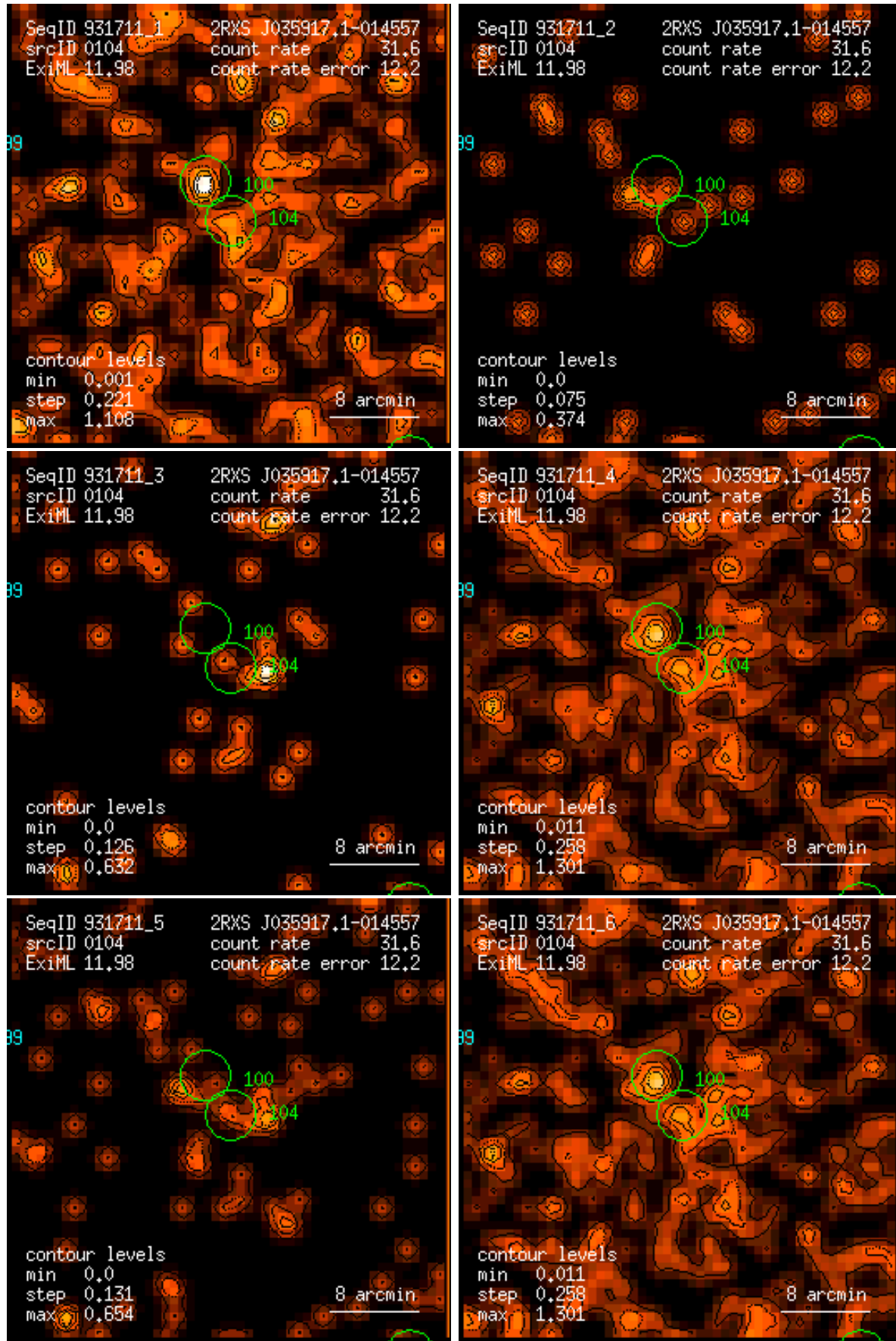
Figure 104: RASS 931711: detection 0104: band rate images, Gaussian filter: (1) PSPC channels 11 – 41, (2) 52 – 90, (3) 91 – 201, (4) 11 – 235, (5) 52 – 201, (6) 11 – 201. Broad band rates in counts/ks. Band rate contour levels in counts/ks/arcmin 2 .
