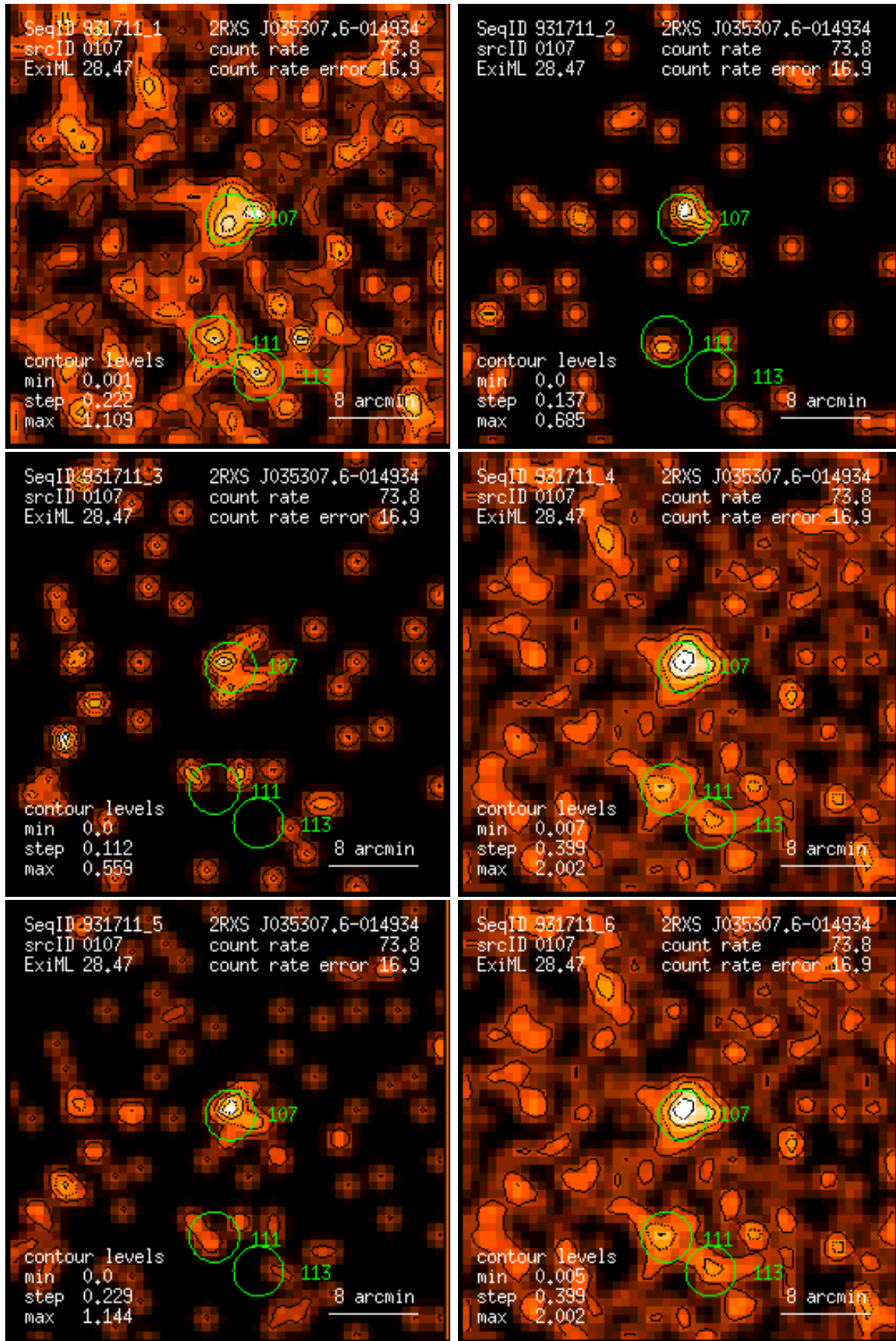
Figure 107: RASS 931711: detection 0107: band rate images, Gaussian filter: (1) PSPC channels 11 – 41, (2) 52 – 90, (3) 91 – 201, (4) 11 – 235, (5) 52 – 201, (6) 11 – 201. Broad band rates in counts/ks. Band rate contour levels in counts/ks/arcmin 2 .
