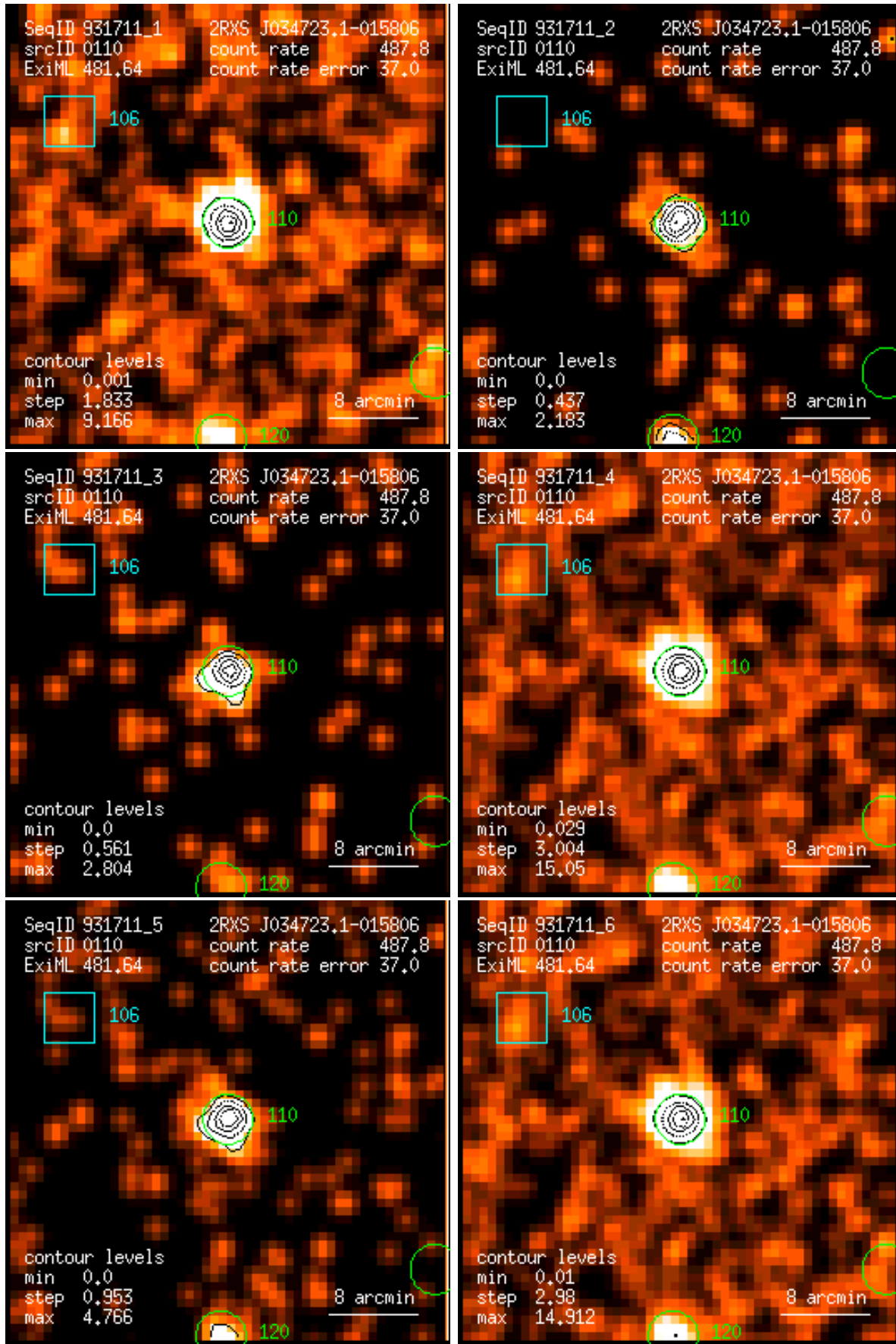
Figure 110: RASS 931711: detection 0110: band rate images, Gaussian filter: (1) PSPC channels 11 – 41, (2) 52 – 90, (3) 91 – 201, (4) 11 – 235, (5) 52 – 201, (6) 11 – 201. Broad band rates in counts/ks. Band rate contour levels in counts/ks/arcmin 2 .
