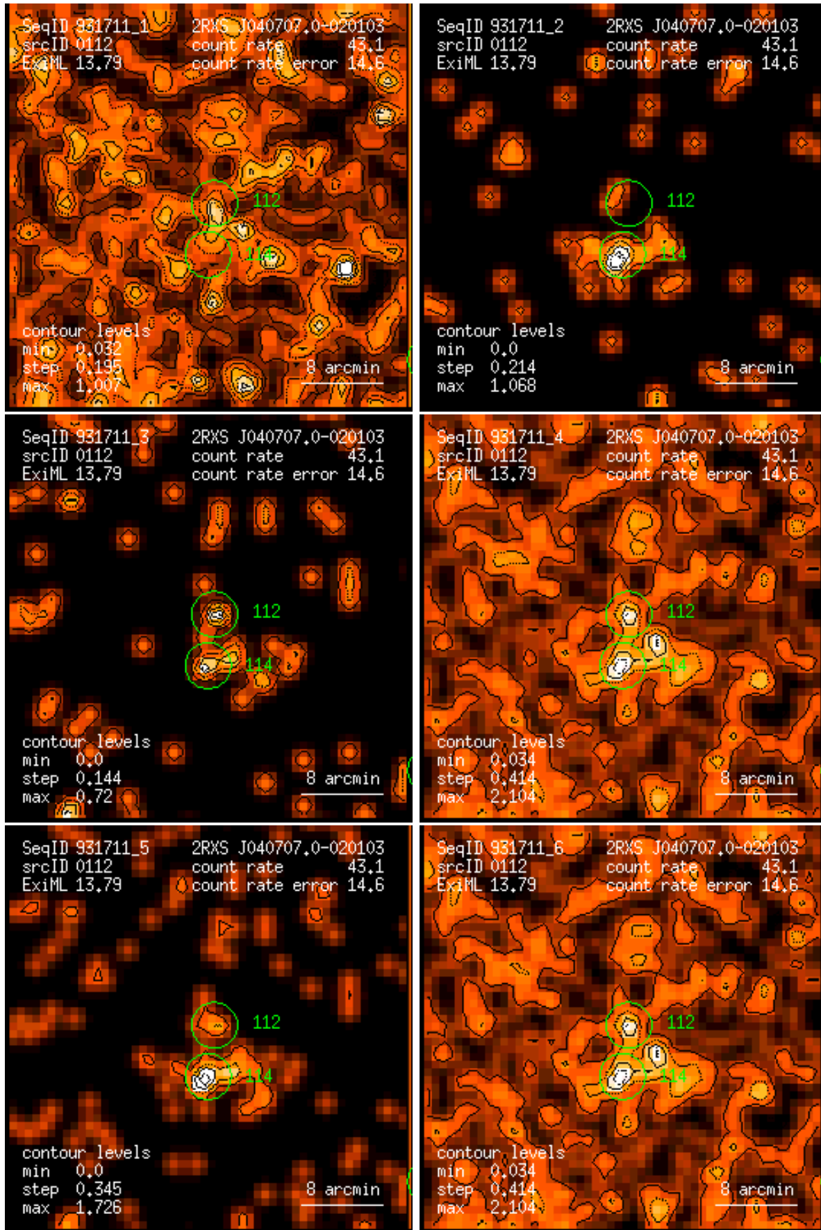
Figure 112: RASS 931711: detection 0112: band rate images, Gaussian filter: (1) PSPC channels 11 – 41, (2) 52 – 90, (3) 91 – 201, (4) 11 – 235, (5) 52 – 201, (6) 11 – 201. Broad band rates in counts/ks. Band rate contour levels in counts/ks/arcmin 2 .
