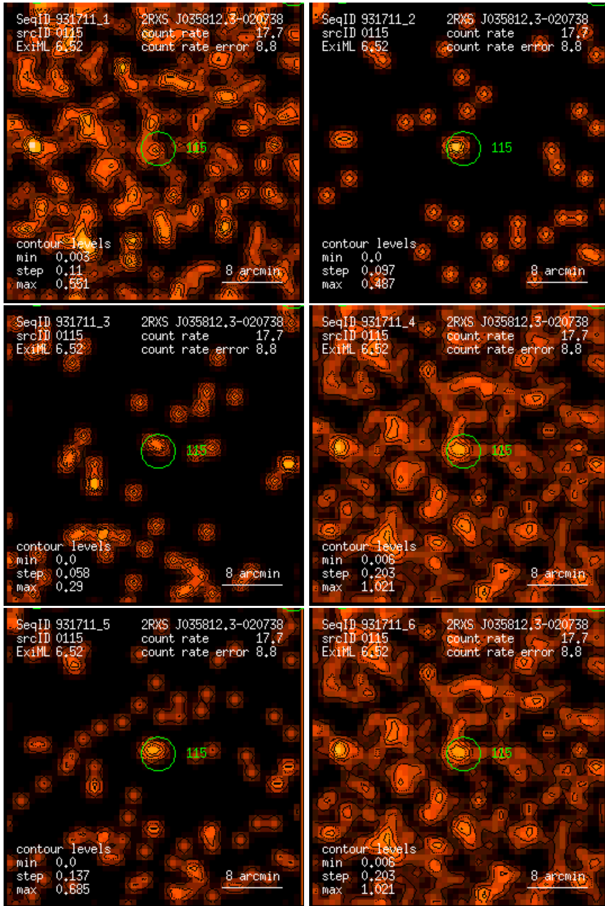
Figure 115: RASS 931711: detection 0115: band rate images, Gaussian filter: (1) PSPC channels 11 – 41, (2) 52 – 90, (3) 91 – 201, (4) 11 – 235, (5) 52 – 201, (6) 11 – 201. Broad band rates in counts/ks. Band rate contour levels in counts/ks/arcmin 2 .
